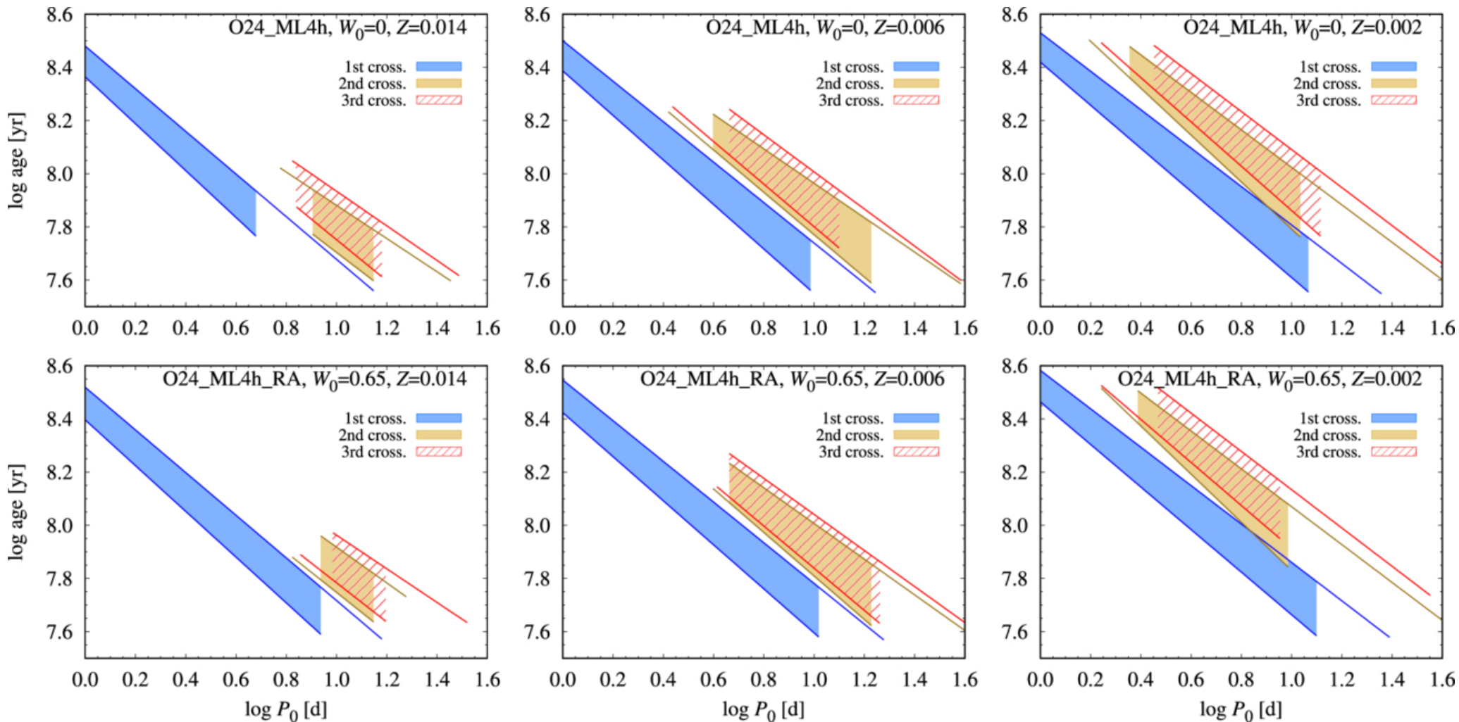
Figure 8. from Radoslaw Smolec et al 2026 Astrophys. J. Suppl. 285 doi:10.3847/1538-4365/ae6ef3 https://dx.doi.org/10.3847/1538-4365/ae6ef3
