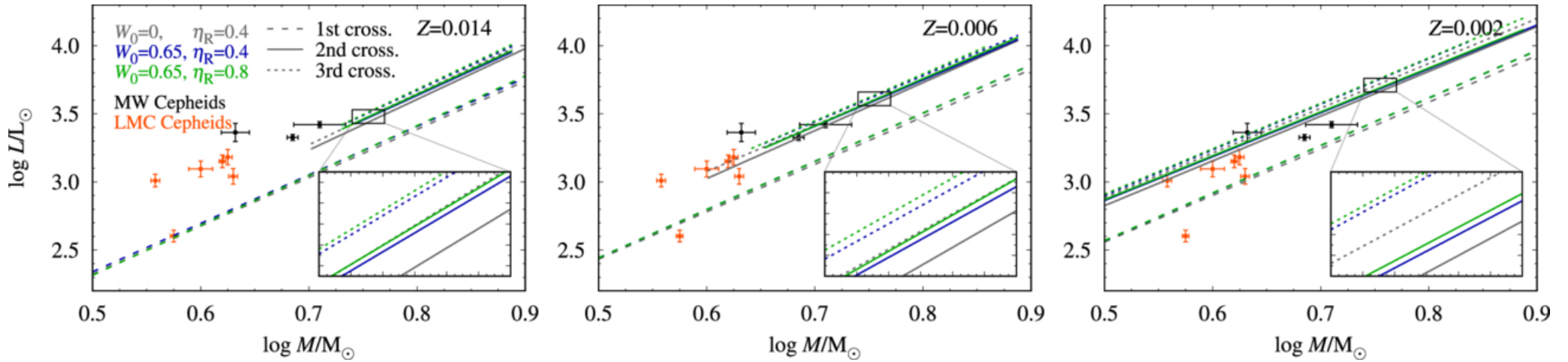
Figure 5. from Radoslaw Smolec et al 2026 Astrophys. J. Suppl. 285 doi:10.3847/1538-4365/ae6ef3 https://dx.doi.org/10.3847/1538-4365/ae6ef3 © 2026. The Author(s). Published by the American Astronomical Society.
