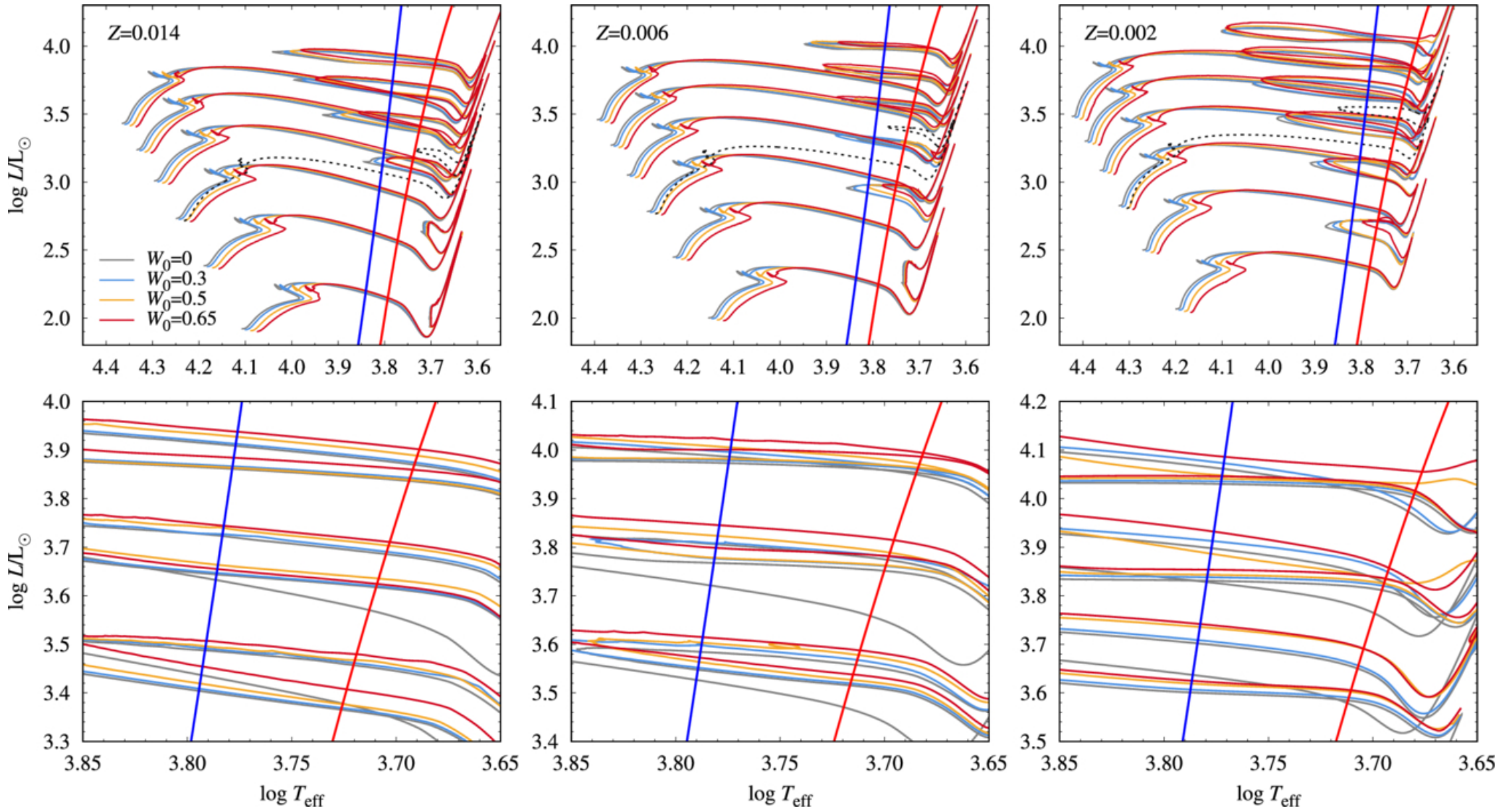
Figure 1. from Radoslaw Smolec et al 2026 Astrophys. J. Suppl. 285 doi:10.3847/1538-4365/ae6ef3 https://dx.doi.org/10.3847/1538-4365/ae6ef3 © 2026. The Author(s). Published by the American Astronomical Society.
