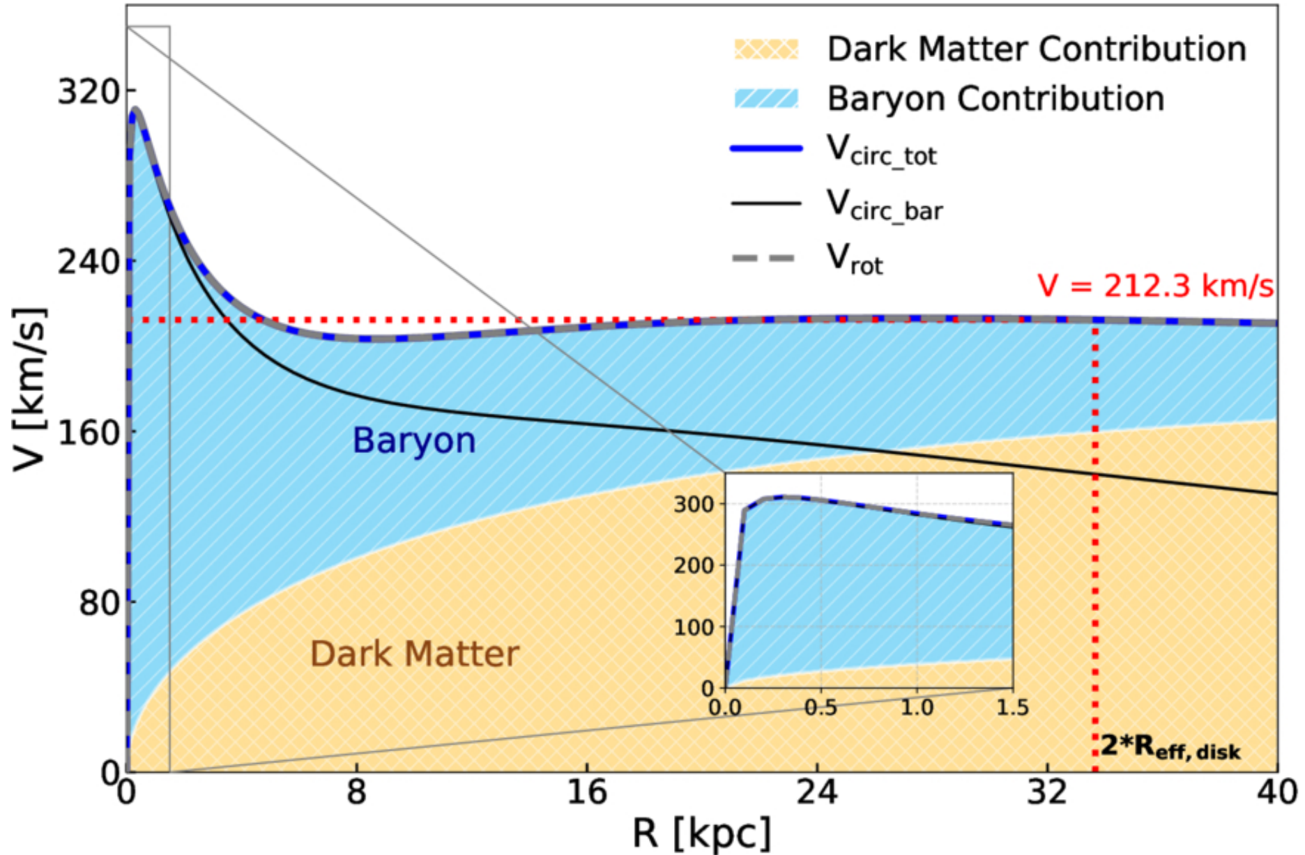
Figure 8. from Ruitian Li et al 2026 Astrophys. J. Suppl. 285 doi:10.3847/1538-4365/ae6ef1 https://dx.doi.org/10.3847/1538-4365/ae6ef1 © 2026. The Author(s). Published by the American Astronomical Society.
