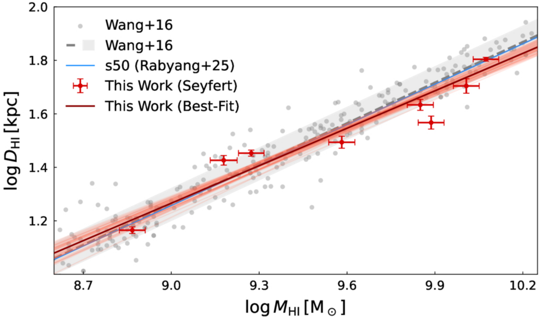
Figure 4. from Ruitian Li et al 2026 Astrophys. J. Suppl. 285 doi:10.3847/1538-4365/ae6ef1 https://dx.doi.org/10.3847/1538-4365/ae6ef1 © 2026. The Author(s). Published by the American Astronomical Society.
