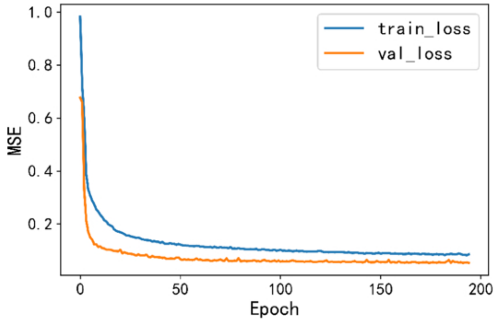
Figure 7. from Shi-Qi Liu et al 2026 Astrophys. J. Suppl. 285 doi:10.3847/1538-4365/ae6eee https://dx.doi.org/10.3847/1538-4365/ae6eee © 2026. The Author(s). Published by the American Astronomical Society.
