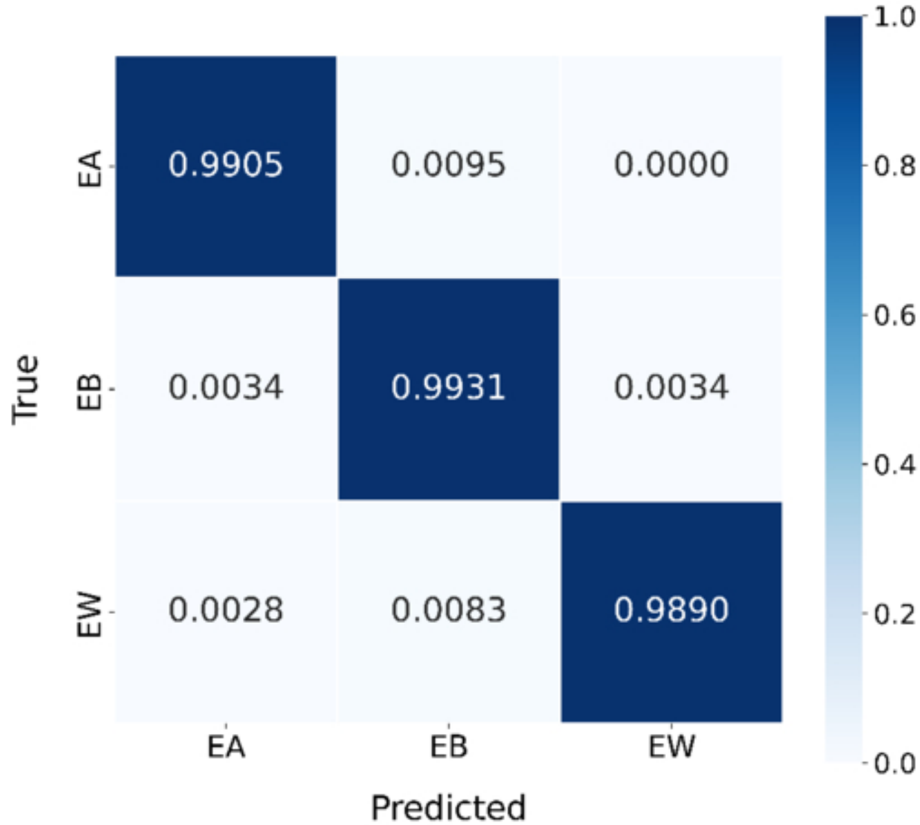
Figure 6. from Shi-Qi Liu et al 2026 Astrophys. J. Suppl. 285 doi:10.3847/1538-4365/ae6eee https://dx.doi.org/10.3847/1538-4365/ae6eee © 2026. The Author(s). Published by the American Astronomical Society.
