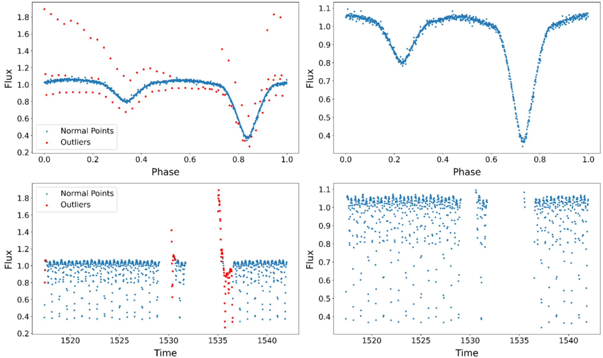
Figure 3. from Shi-Qi Liu et al 2026 Astrophys. J. Suppl. 285 doi:10.3847/1538-4365/ae6eee https://dx.doi.org/10.3847/1538-4365/ae6eee © 2026. The Author(s). Published by the American Astronomical Society.
