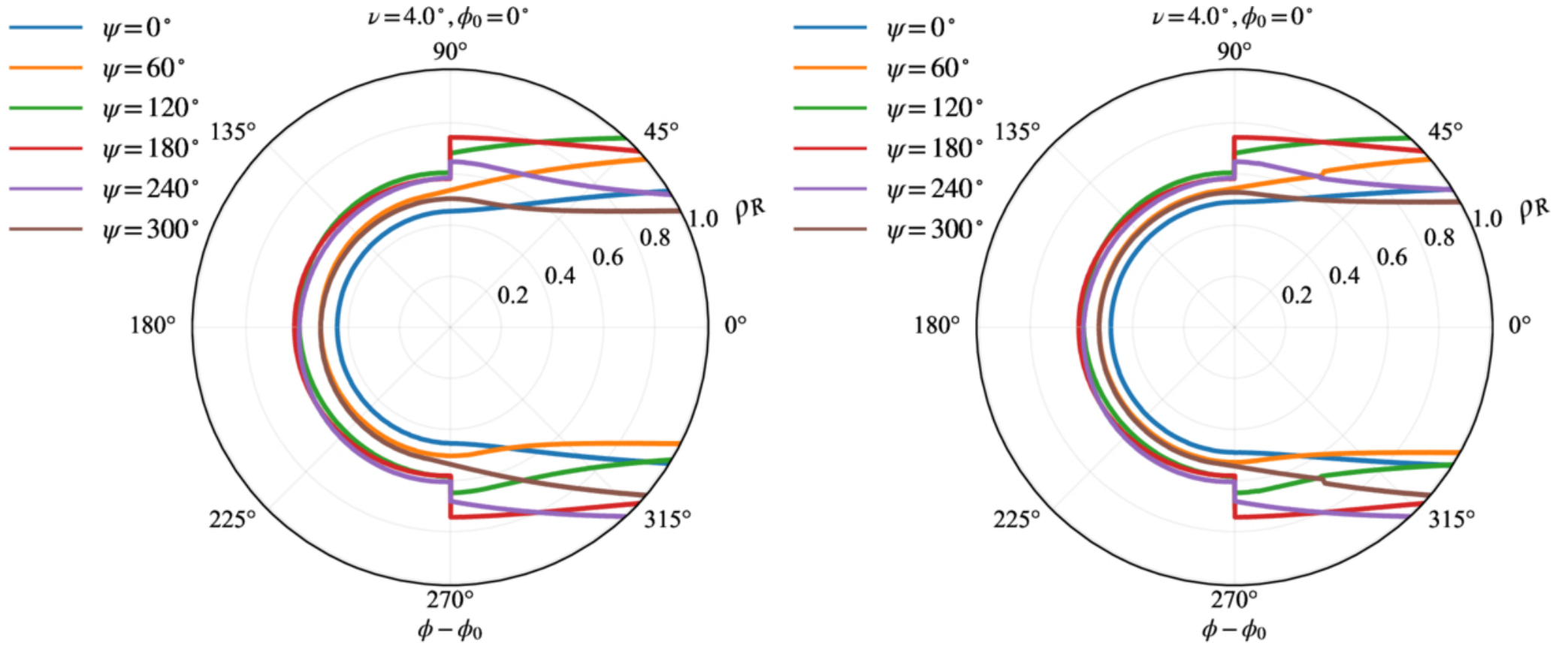
Figure 6. from Markus Gaug et al 2026 Astrophys. J. Suppl. 285 doi:10.3847/1538-4365/ae6da5 https://dx.doi.org/10.3847/1538-4365/ae6da5
