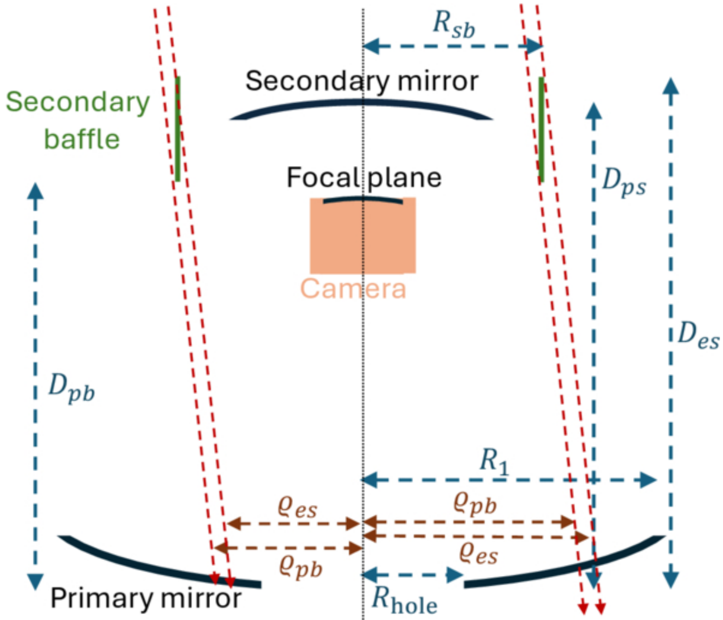
Figure 4. from Markus Gaug et al 2026 Astrophys. J. Suppl. 285 doi:10.3847/1538-4365/ae6da5 https://dx.doi.org/10.3847/1538-4365/ae6da5 © 2026. The Author(s). Published by the American Astronomical Society.
