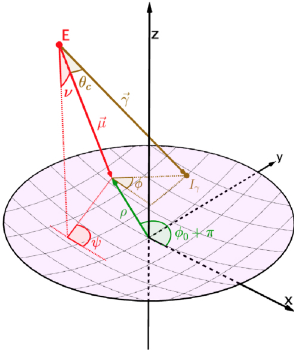
Figure 1. from Markus Gaug et al 2026 Astrophys. J. Suppl. 285 doi:10.3847/1538-4365/ae6da5 https://dx.doi.org/10.3847/1538-4365/ae6da5 © 2026. The Author(s). Published by the American Astronomical Society.
