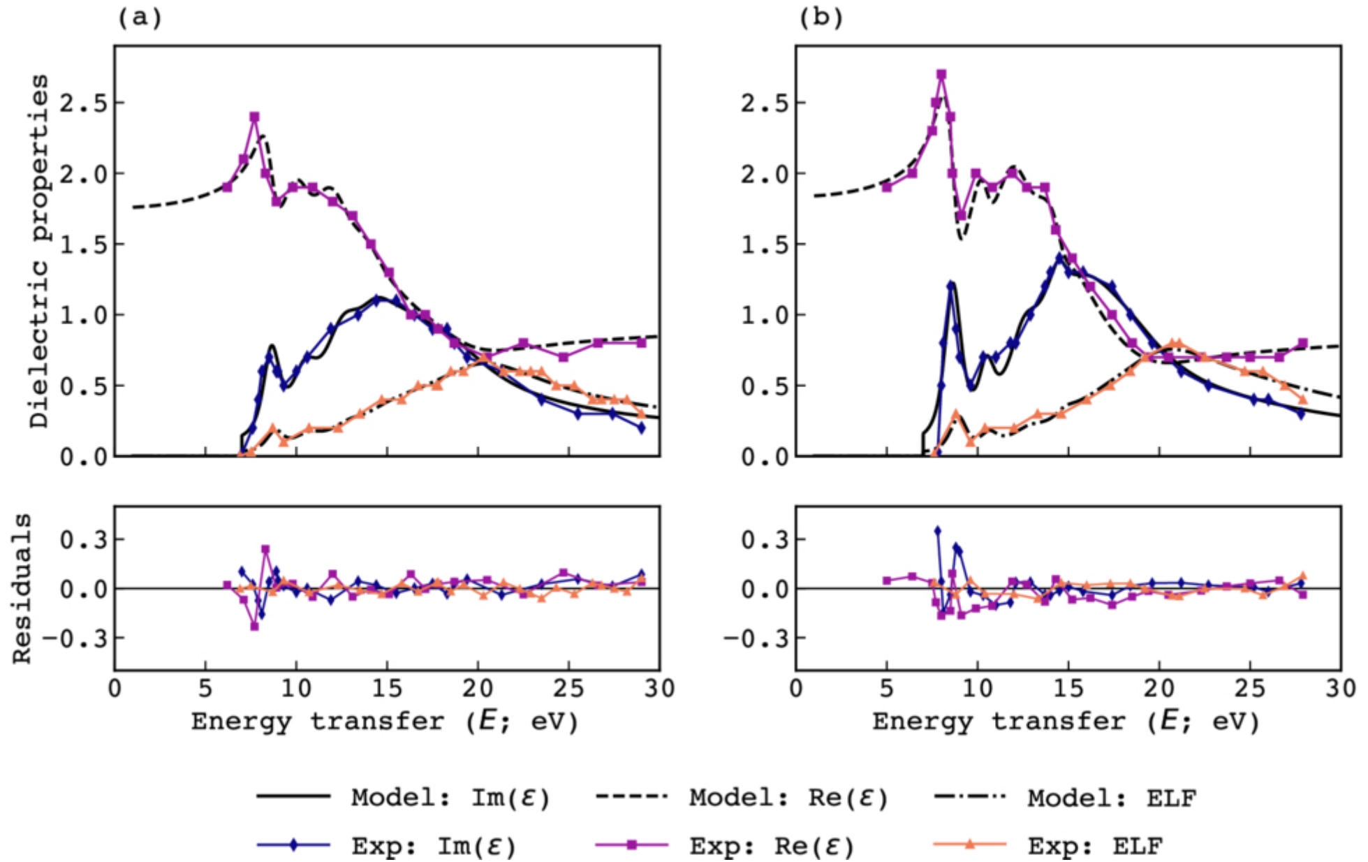
Figure 4. from Gideon Yoffe et al 2026 Astrophys. J. Suppl. 284 doi:10.3847/1538-4365/ae6b7a https://dx.doi.org/10.3847/1538-4365/ae6b7a © 2026. The Author(s). Published by the American Astronomical Society.
