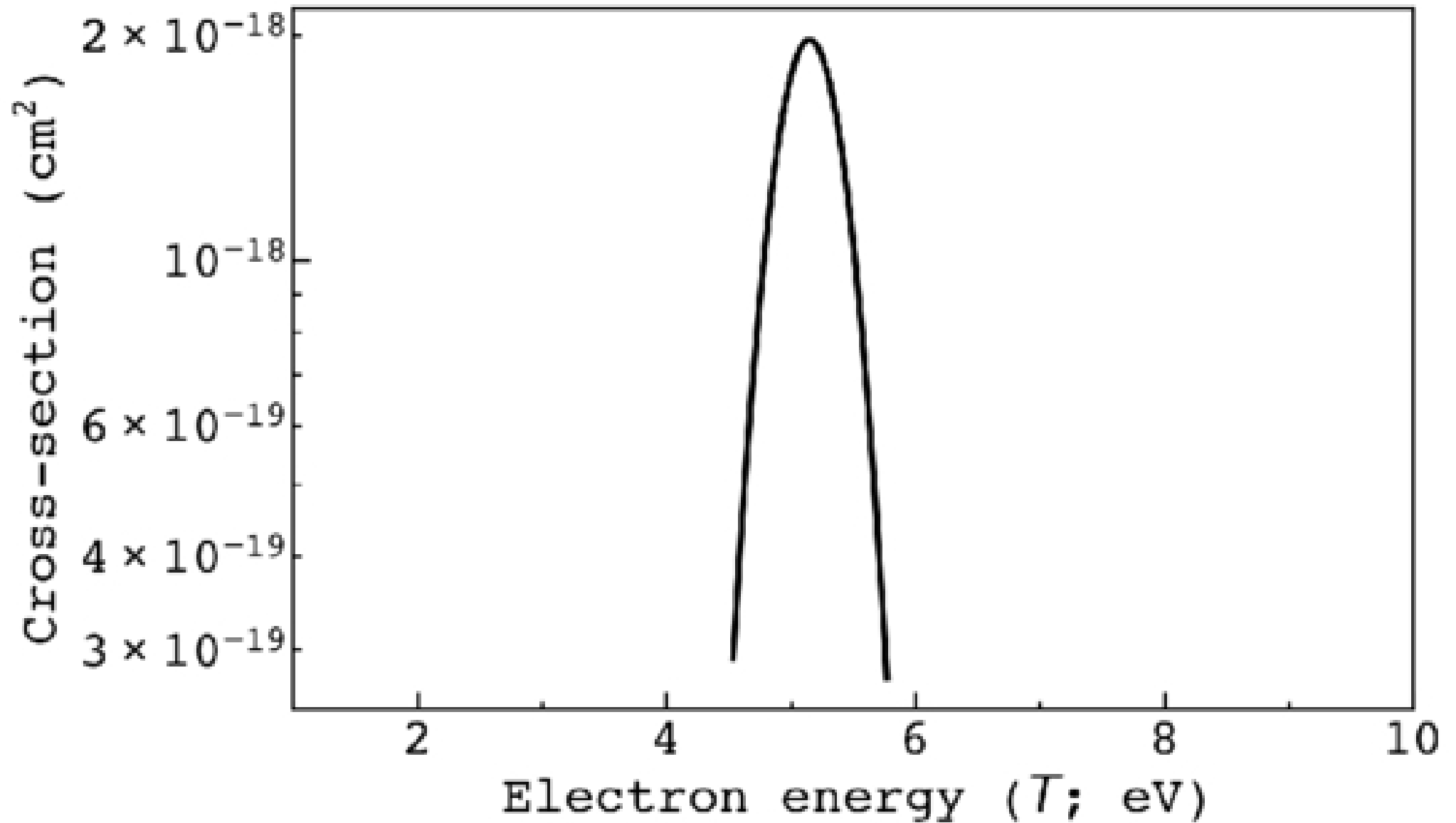
Figure 3. from Gideon Yoffe et al 2026 Astrophys. J. Suppl. 284 doi:10.3847/1538-4365/ae6b7a https://dx.doi.org/10.3847/1538-4365/ae6b7a © 2026. The Author(s). Published by the American Astronomical Society.
