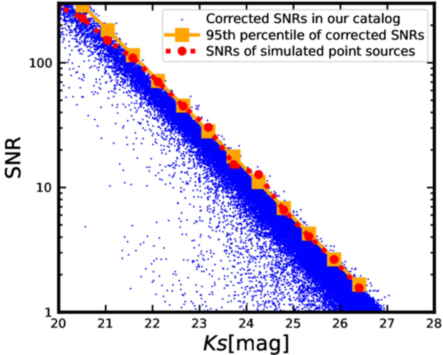
Figure 7. from Hanwen Sun et al 2026 Astrophys. J. Suppl. 285 doi:10.3847/1538-4365/ae69d2 https://dx.doi.org/10.3847/1538-4365/ae69d2 © 2026. The Author(s). Published by the American Astronomical Society.
