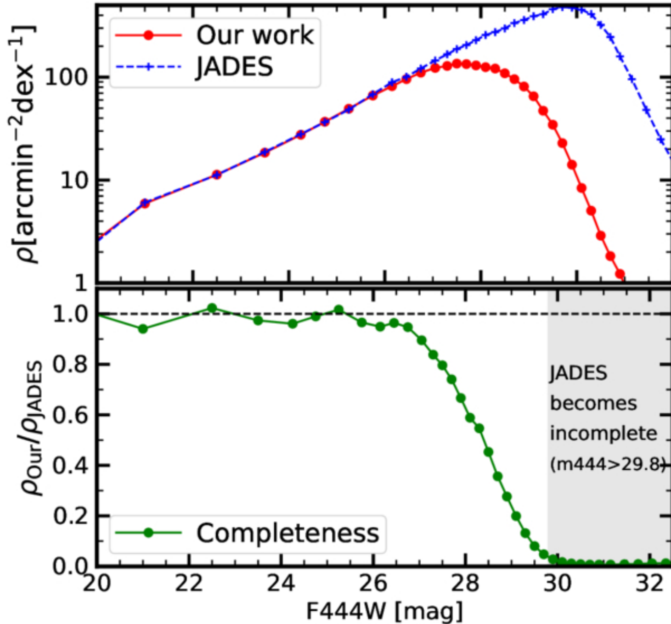
Figure 5. from Hanwen Sun et al 2026 Astrophys. J. Suppl. 285 doi:10.3847/1538-4365/ae69d2 https://dx.doi.org/10.3847/1538-4365/ae69d2 © 2026. The Author(s). Published by the American Astronomical Society.
