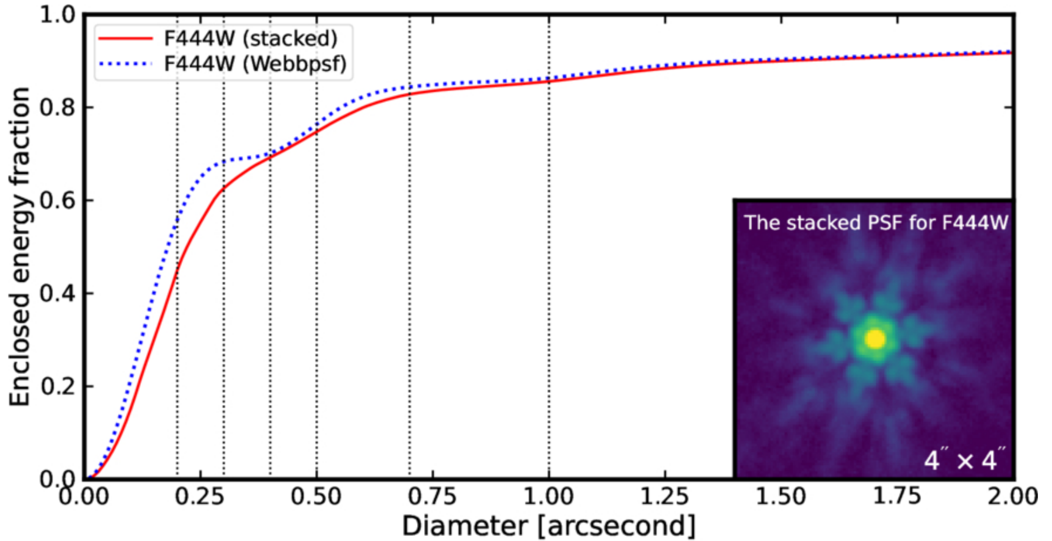
Figure 4. from Hanwen Sun et al 2026 Astrophys. J. Suppl. 285 doi:10.3847/1538-4365/ae69d2 https://dx.doi.org/10.3847/1538-4365/ae69d2 © 2026. The Author(s). Published by the American Astronomical Society.
