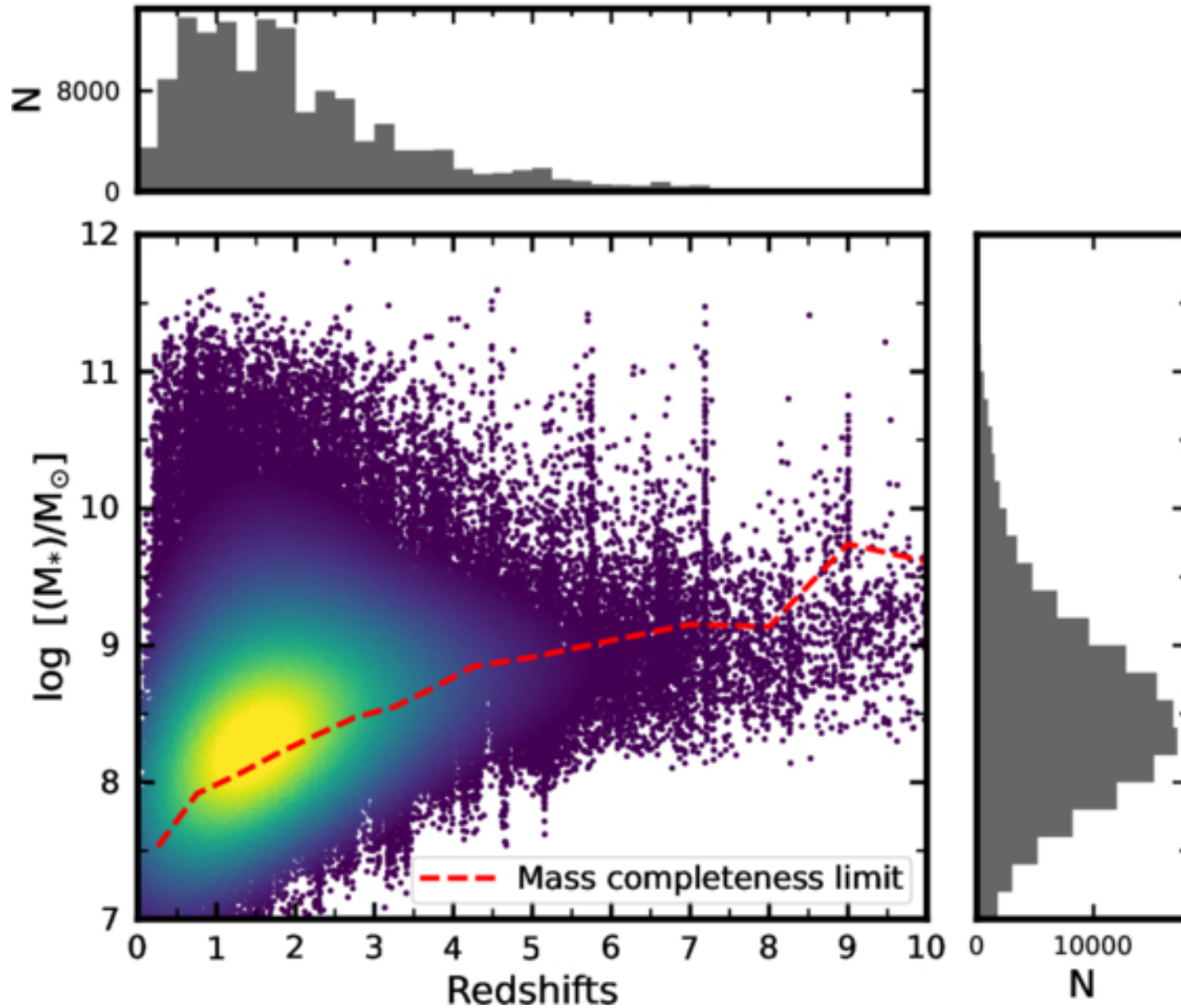
Figure 10. from Hanwen Sun et al 2026 Astrophys. J. Suppl. 285 doi:10.3847/1538-4365/ae69d2 https://dx.doi.org/10.3847/1538-4365/ae69d2 © 2026. The Author(s). Published by the American Astronomical Society.
