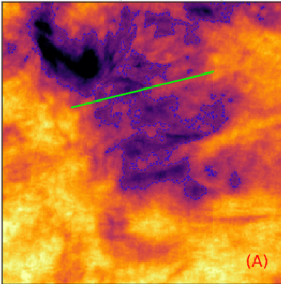
Chromospheric Intensity
