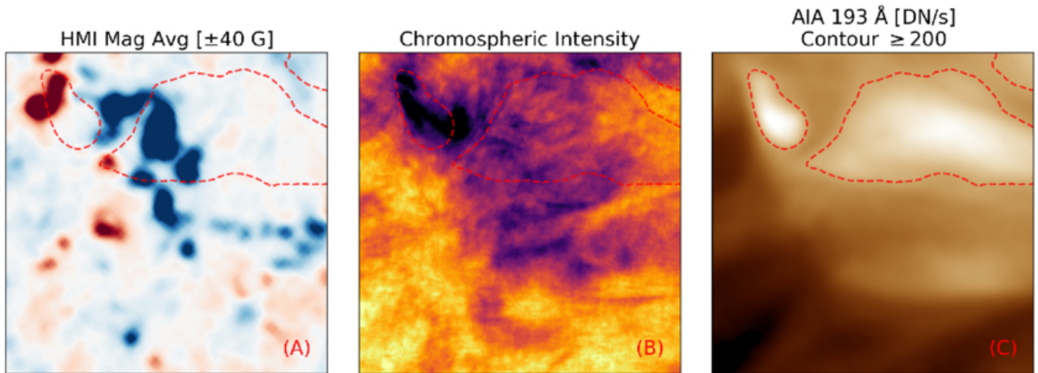
Figure 8. from Huaiming Li et al 2026 Astrophys. J. Suppl. 284 doi:10.3847/1538-4365/ae6911 https://dx.doi.org/10.3847/1538-4365/ae6911 © 2026. The Author(s). Published by the American Astronomical Society.
