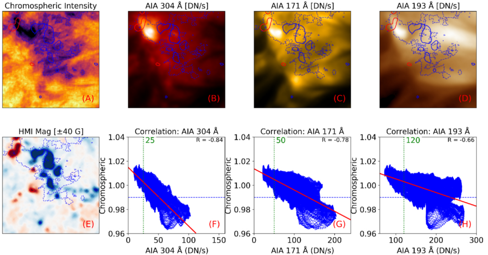
Figure 7. from Huaiming Li et al 2026 Astrophys. J. Suppl. 284 doi:10.3847/1538-4365/ae6911 https://dx.doi.org/10.3847/1538-4365/ae6911 © 2026. The Author(s). Published by the American Astronomical Society.
