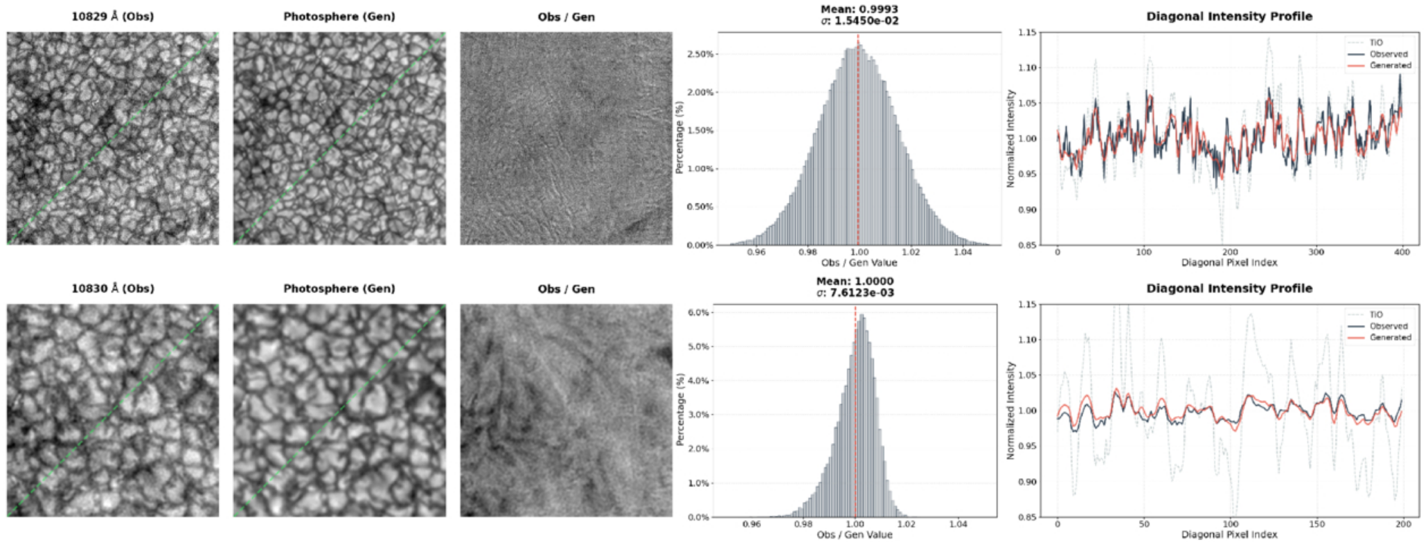
Figure 4. from Huaiming Li et al 2026 Astrophys. J. Suppl. 284 doi:10.3847/1538-4365/ae6911 https://dx.doi.org/10.3847/1538-4365/ae6911 © 2026. The Author(s). Published by the American Astronomical Society.
