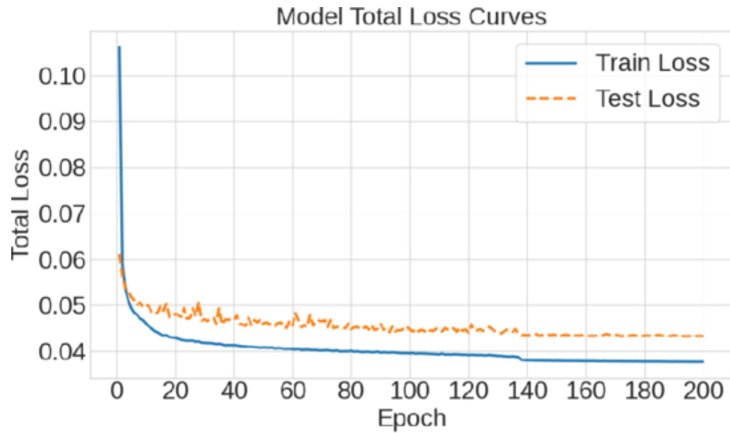
(a) Model A Loss
