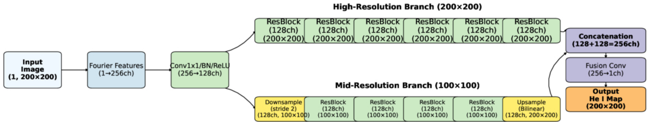
Figure 13. from Huaiming Li et al 2026 Astrophys. J. Suppl. 284 doi:10.3847/1538-4365/ae6911 https://dx.doi.org/10.3847/1538-4365/ae6911 © 2026. The Author(s). Published by the American Astronomical Society.
