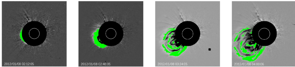
(a) Ours
