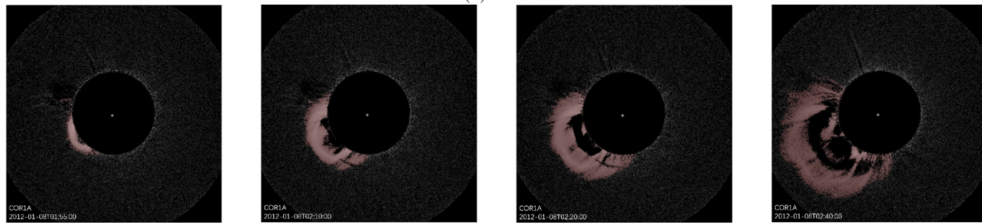
(b) CAMEL2
