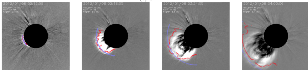
(c) SEEDS
