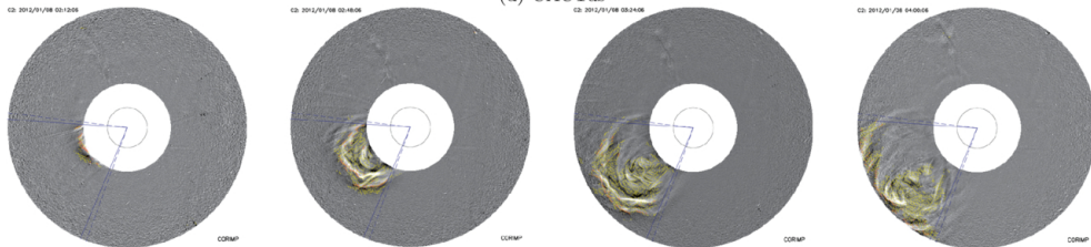
(e) CORIMP
