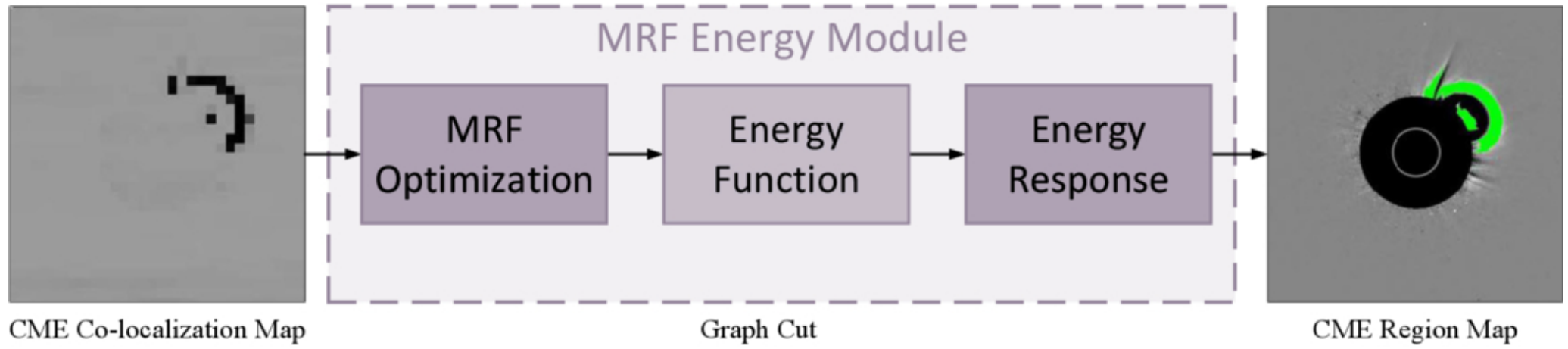
Figure 5. from Peican He et al 2026 Astrophys. J. Suppl. 284 doi:10.3847/1538-4365/ae66e6 https://dx.doi.org/10.3847/1538-4365/ae66e6 © 2026. The Author(s). Published by the American Astronomical Society.
