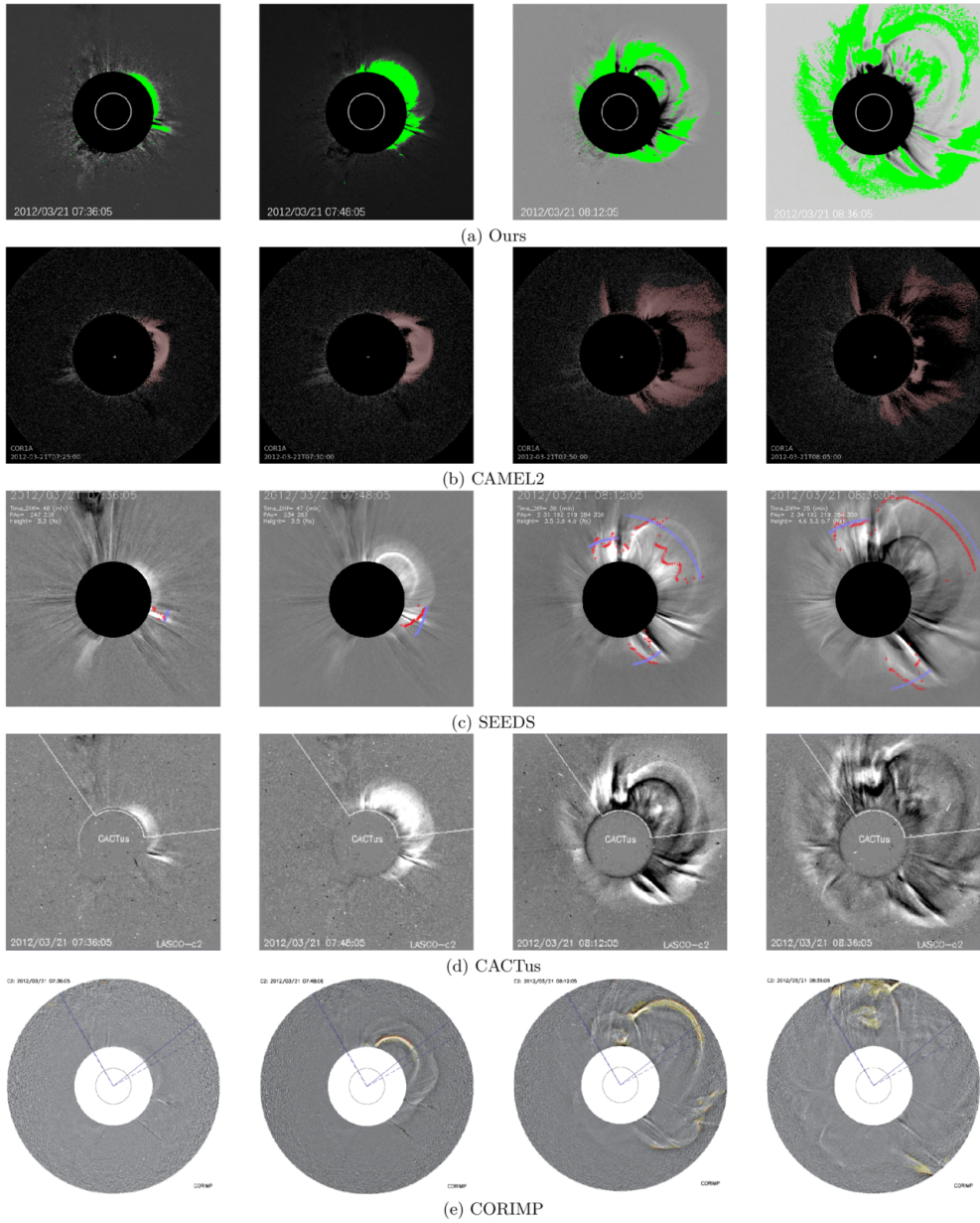
Figure 10. from Peican He et al 2026 Astrophys. J. Suppl. 284 doi:10.3847/1538-4365/ae66e6 https://dx.doi.org/10.3847/1538-4365/ae66e6 © 2026. The Author(s). Published by the American Astronomical Society.
