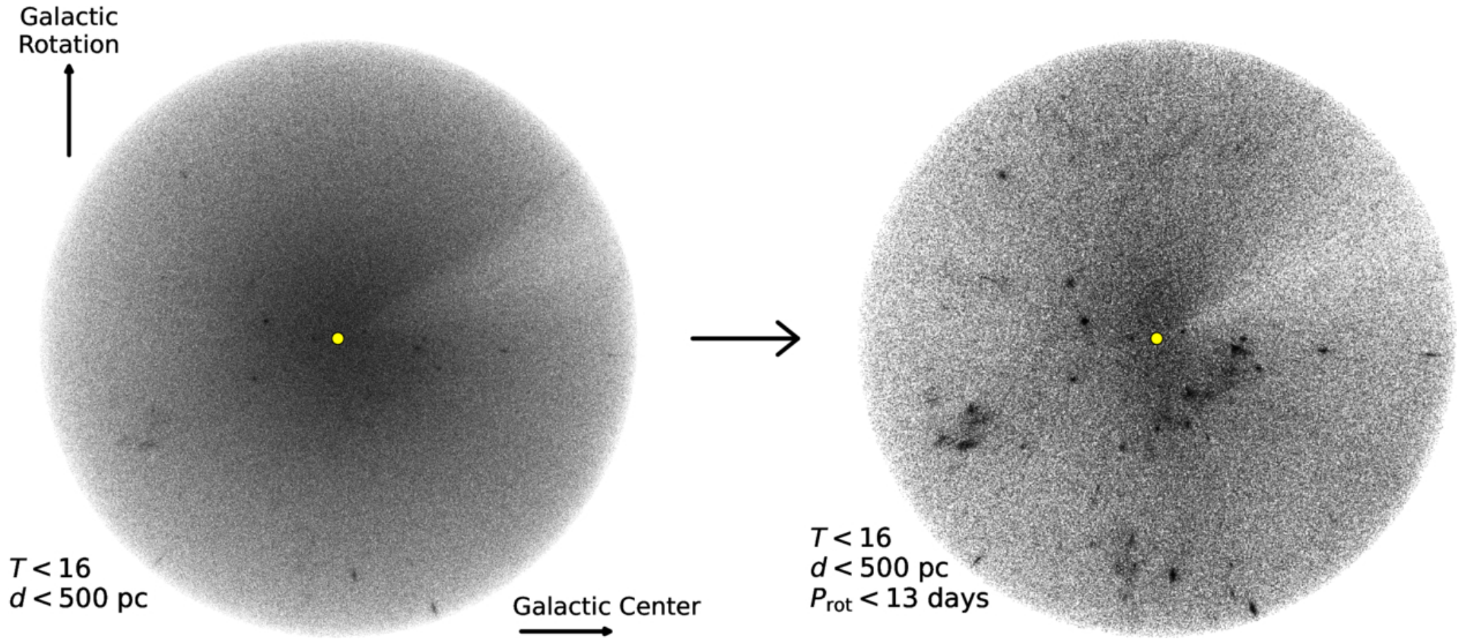
Figure 8. from Andrew W. Boyle et al 2026 Astrophys. J. Suppl. 284 doi:10.3847/1538-4365/ae6657 https://dx.doi.org/10.3847/1538-4365/ae6657 © 2026. The Author(s). Published by the American Astronomical Society.
