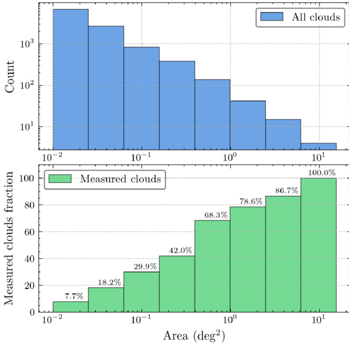
Figure 8. from Juan Mei et al 2026 Astrophys. J. Suppl. 284 doi:10.3847/1538-4365/ae6580 https://dx.doi.org/10.3847/1538-4365/ae6580 © 2026. The Author(s). Published by the American Astronomical Society.
