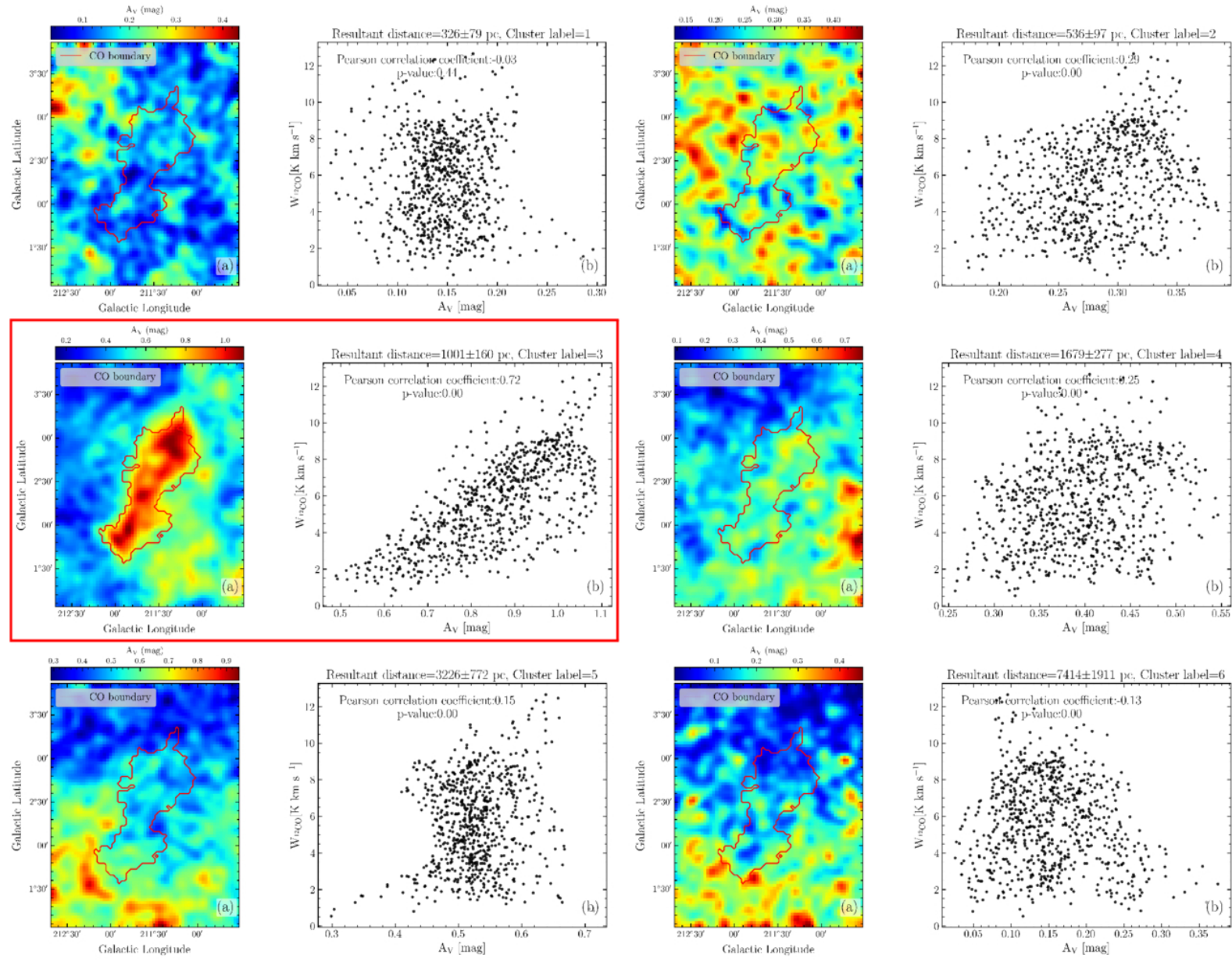
Figure 5. from Juan Mei et al 2026 Astrophys. J. Suppl. 284 doi:10.3847/1538-4365/ae6580 https://dx.doi.org/10.3847/1538-4365/ae6580 © 2026. The Author(s). Published by the American Astronomical Society.
