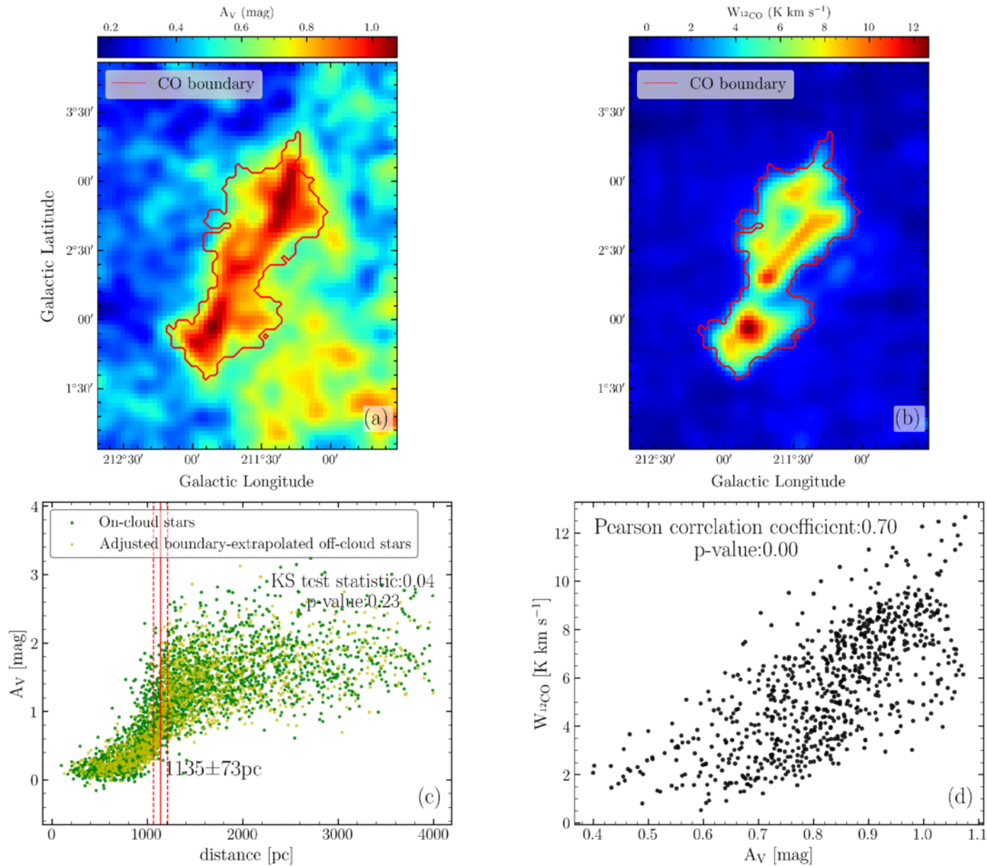
Figure 3. from Juan Mei et al 2026 Astrophys. J. Suppl. 284 doi:10.3847/1538-4365/ae6580 https://dx.doi.org/10.3847/1538-4365/ae6580 © 2026. The Author(s). Published by the American Astronomical Society.
