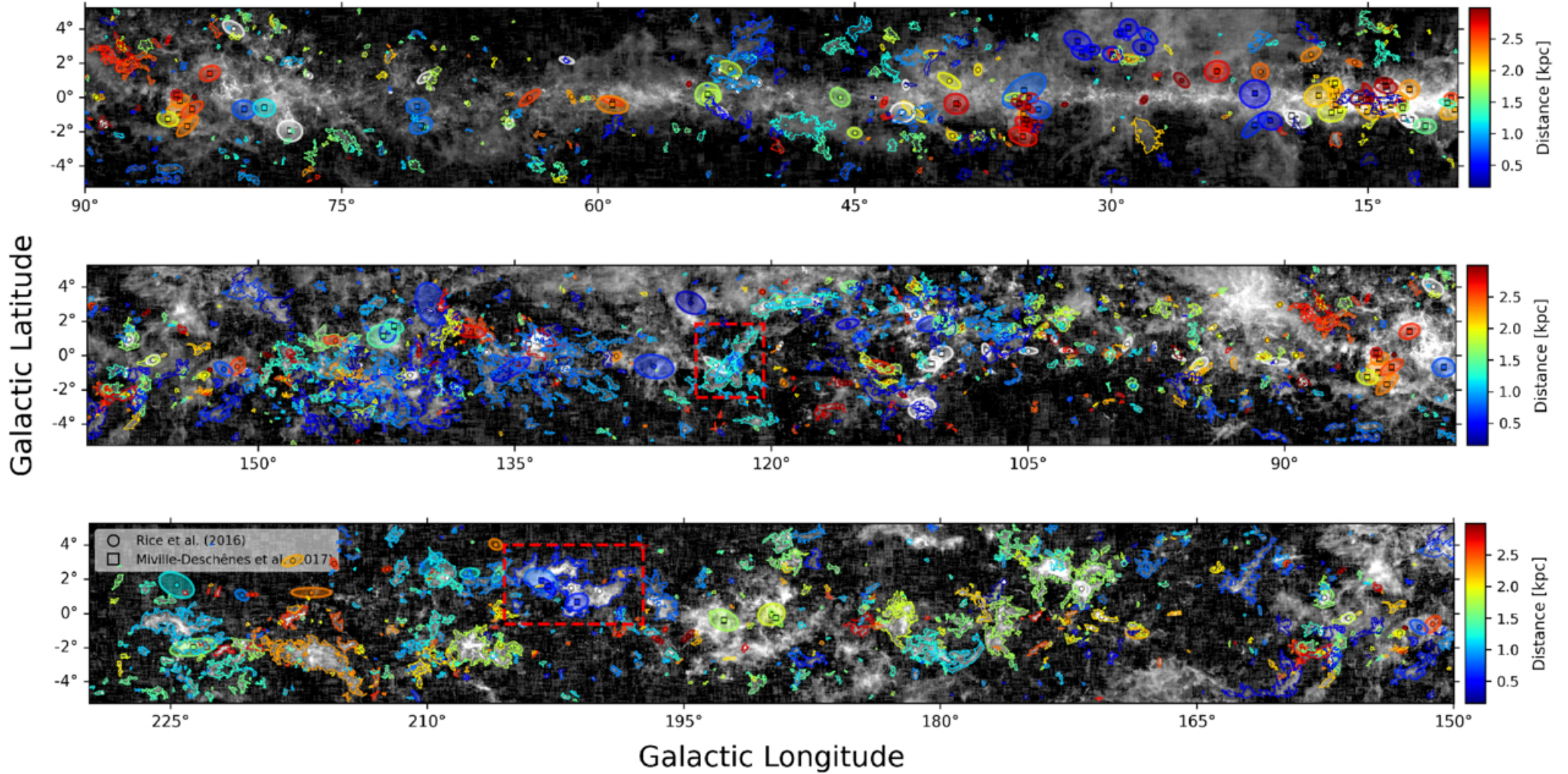
Figure 12. from Juan Mei et al 2026 Astrophys. J. Suppl. 284 doi:10.3847/1538-4365/ae6580 https://dx.doi.org/10.3847/1538-4365/ae6580 © 2026. The Author(s). Published by the American Astronomical Society.
