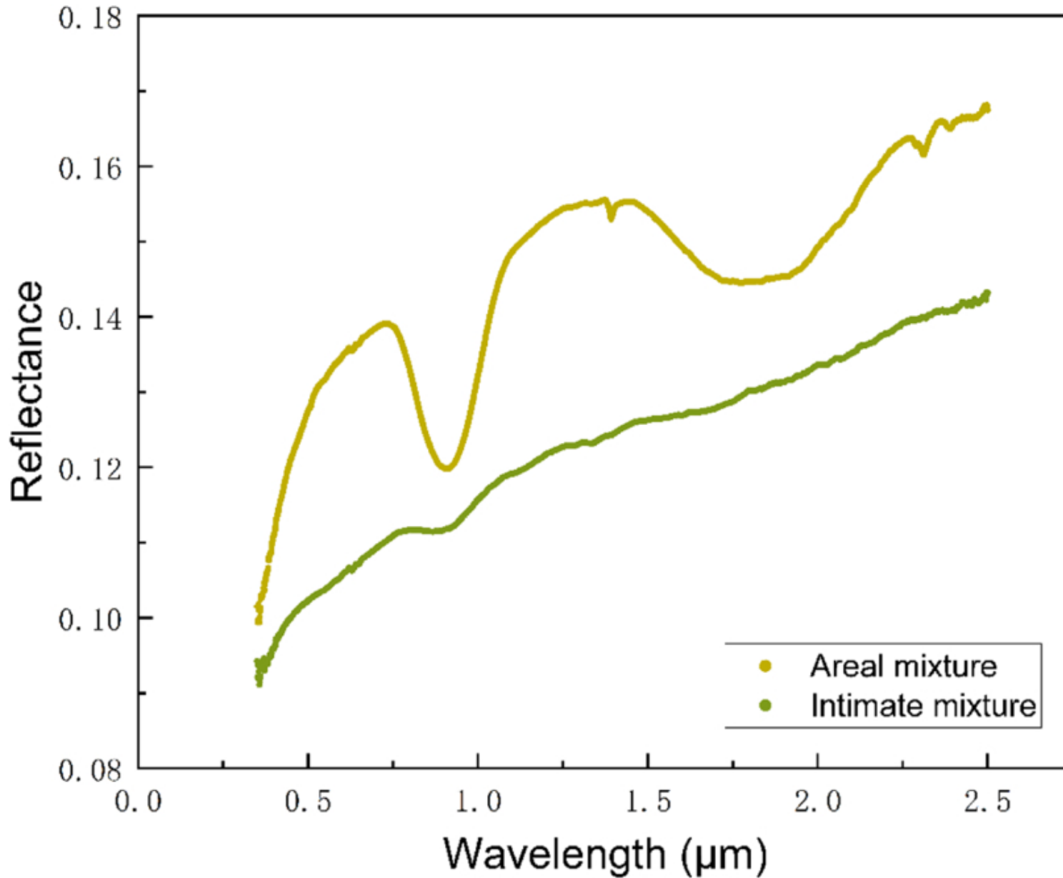
Figure 9. from Pengyue Wang et al 2026 Astrophys. J. Suppl. 284 doi:10.3847/1538-4365/ae644a https://dx.doi.org/10.3847/1538-4365/ae644a © 2026. The Author(s). Published by the American Astronomical Society.
