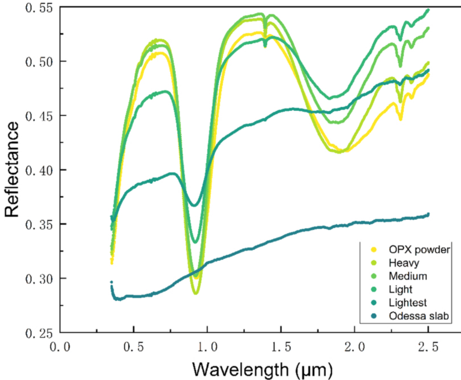
Figure 8. from Pengyue Wang et al 2026 Astrophys. J. Suppl. 284 doi:10.3847/1538-4365/ae644a https://dx.doi.org/10.3847/1538-4365/ae644a © 2026. The Author(s). Published by the American Astronomical Society.
