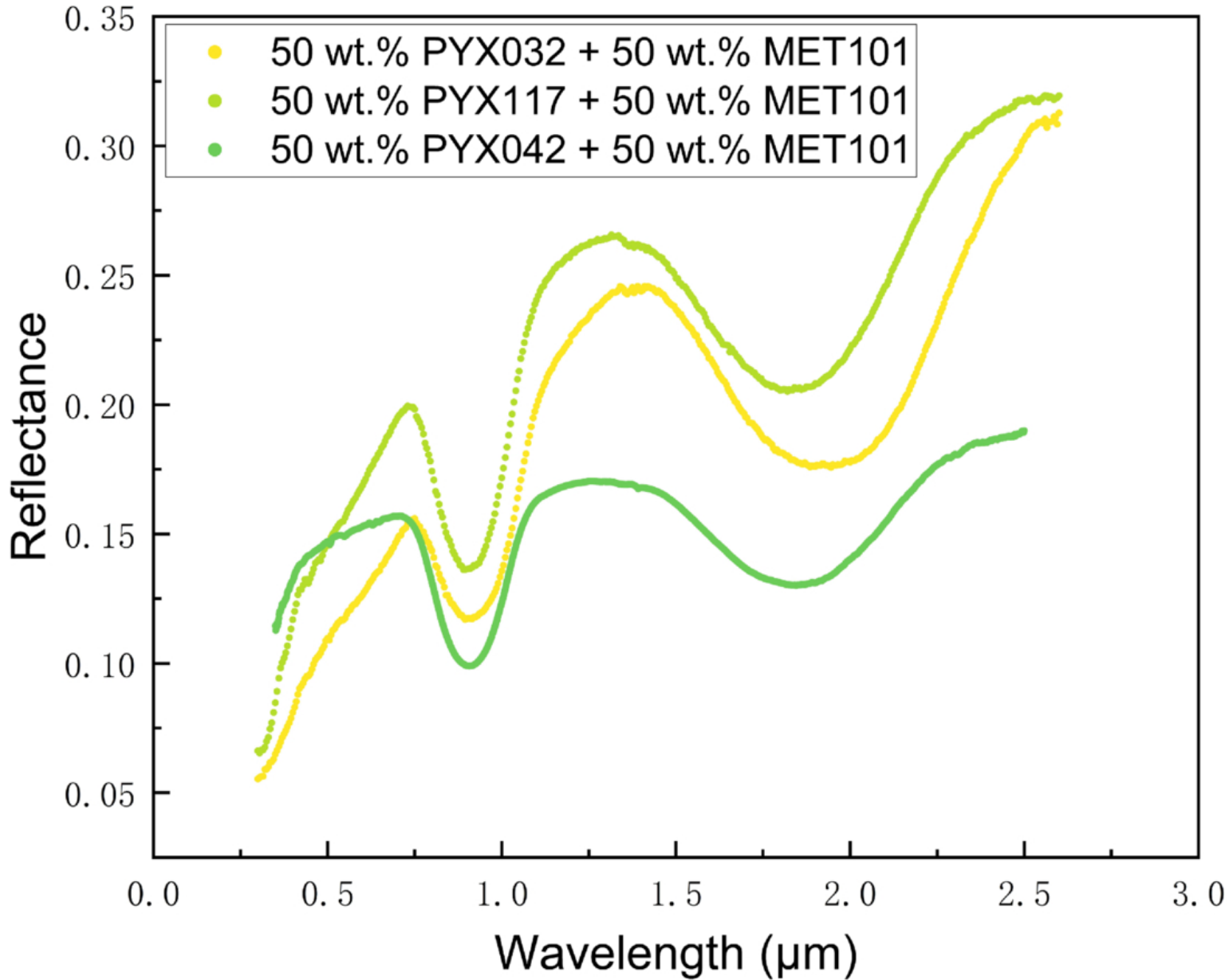
Figure 4. from Pengyue Wang et al 2026 Astrophys. J. Suppl. 284 doi:10.3847/1538-4365/ae644a https://dx.doi.org/10.3847/1538-4365/ae644a © 2026. The Author(s). Published by the American Astronomical Society.
