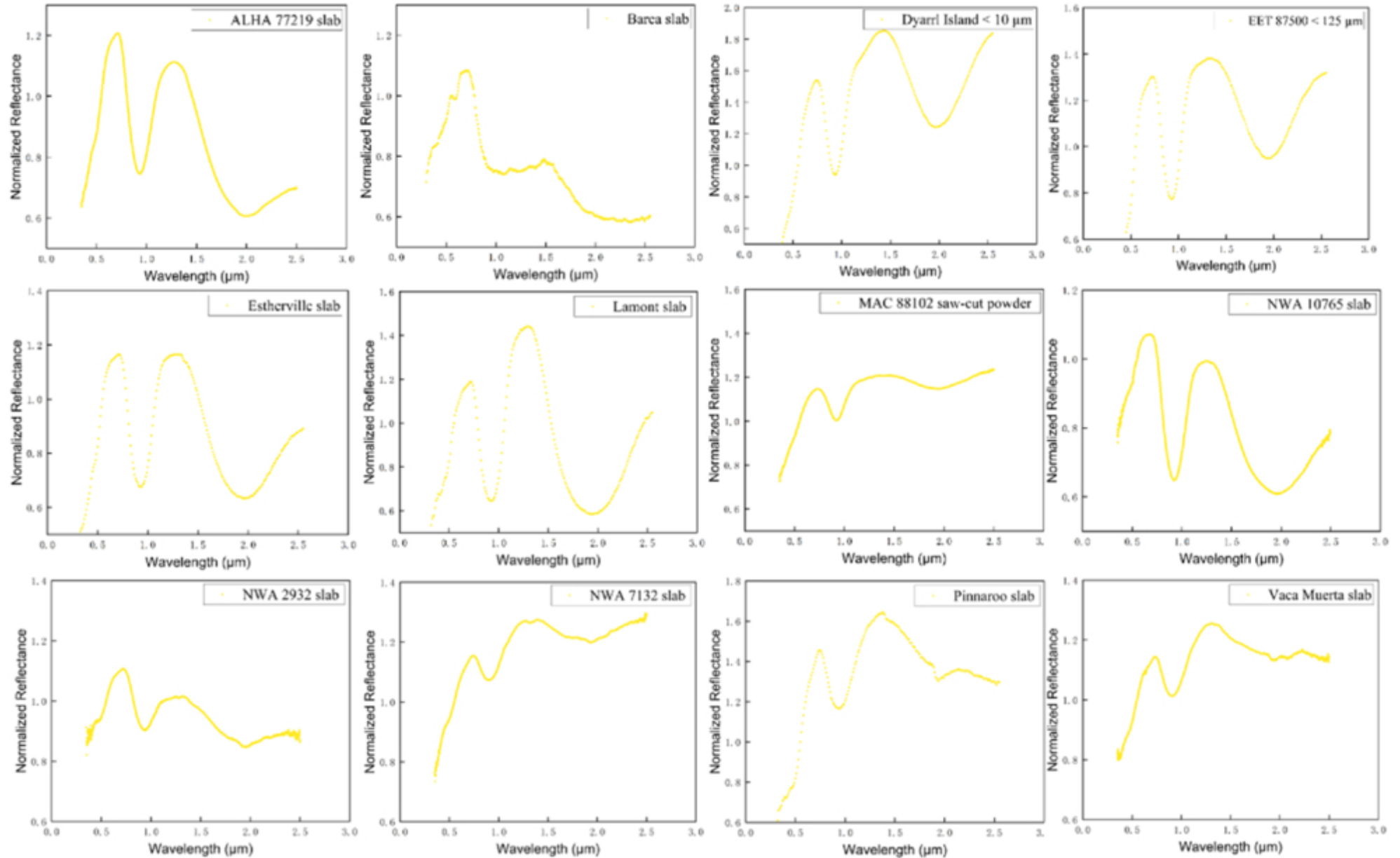
Figure 12. from Pengyue Wang et al 2026 Astrophys. J. Suppl. 284 doi:10.3847/1538-4365/ae644a https://dx.doi.org/10.3847/1538-4365/ae644a © 2026. The Author(s). Published by the American Astronomical Society.
