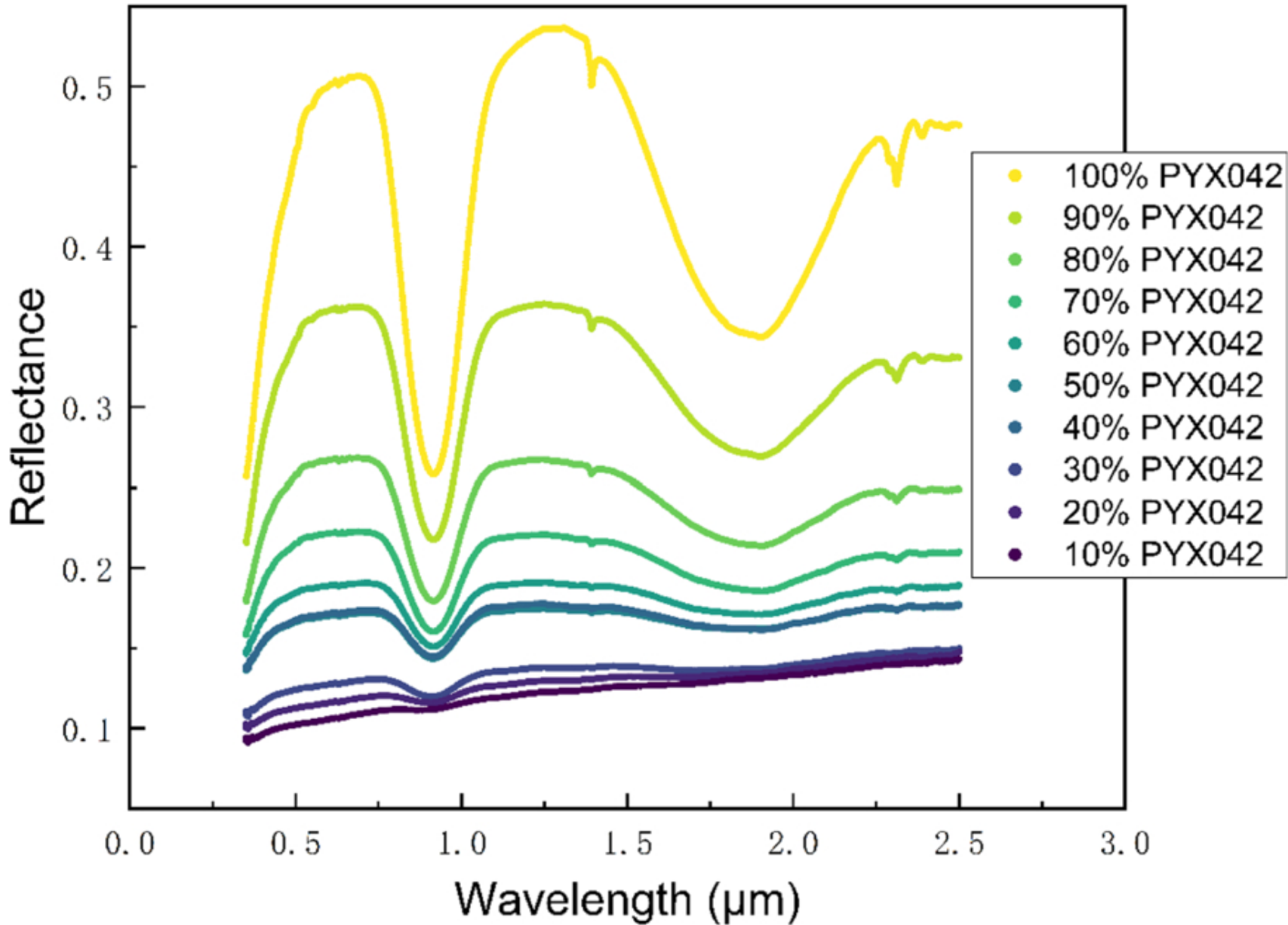
Figure 10. from Pengyue Wang et al 2026 Astrophys. J. Suppl. 284 doi:10.3847/1538-4365/ae644a https://dx.doi.org/10.3847/1538-4365/ae644a © 2026. The Author(s). Published by the American Astronomical Society.
