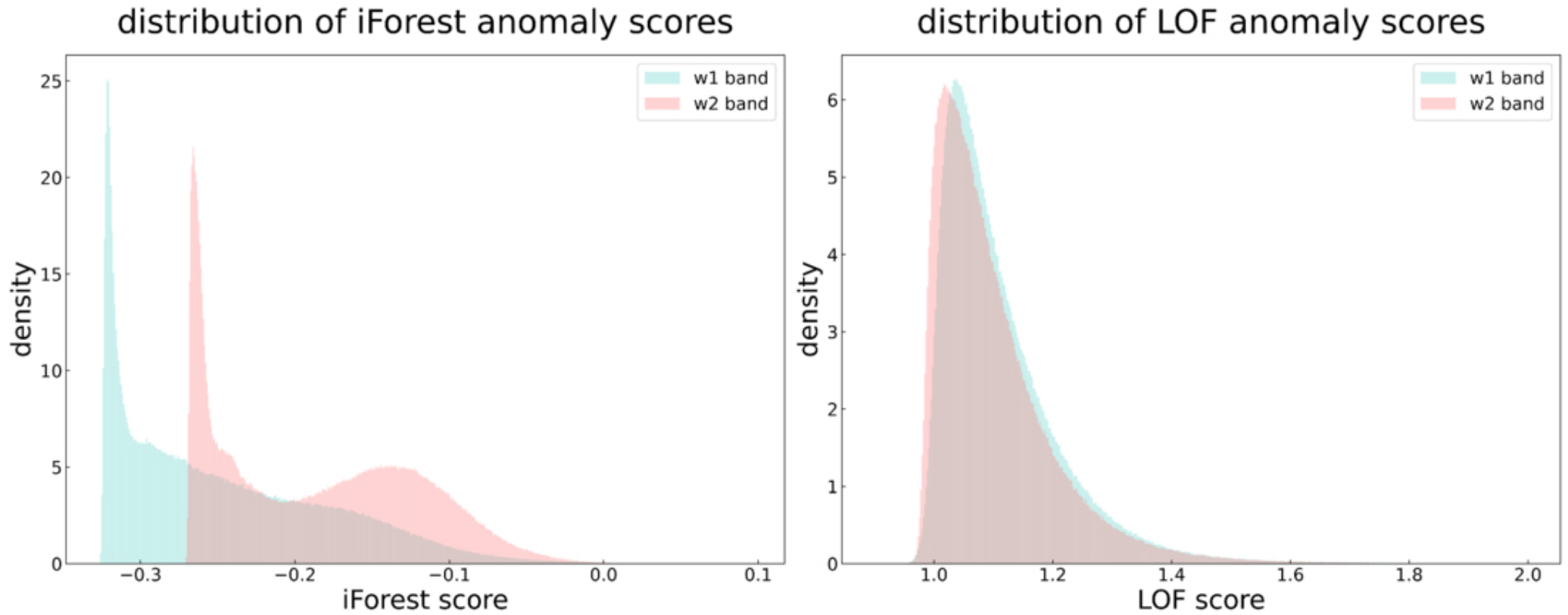
Figure 8. from Zihan Kang et al 2026 Astrophys. J. Suppl. 284 doi:10.3847/1538-4365/ae623c https://dx.doi.org/10.3847/1538-4365/ae623c © 2026. The Author(s). Published by the American Astronomical Society.
