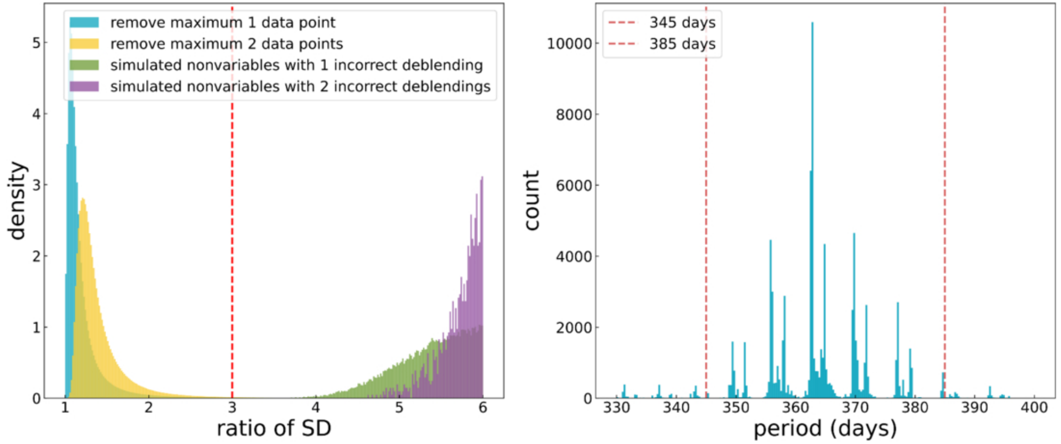
Figure 5. from Zihan Kang et al 2026 Astrophys. J. Suppl. 284 doi:10.3847/1538-4365/ae623c https://dx.doi.org/10.3847/1538-4365/ae623c © 2026. The Author(s). Published by the American Astronomical Society.
