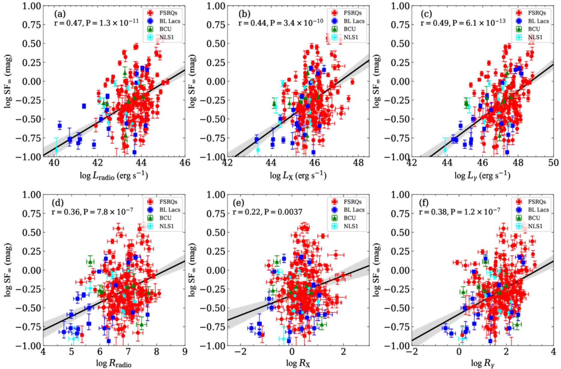
Figure 5. from Yongyun Chen et al 2026 Astrophys. J. Suppl. 284 doi:10.3847/1538-4365/ae6075 https://dx.doi.org/10.3847/1538-4365/ae6075
