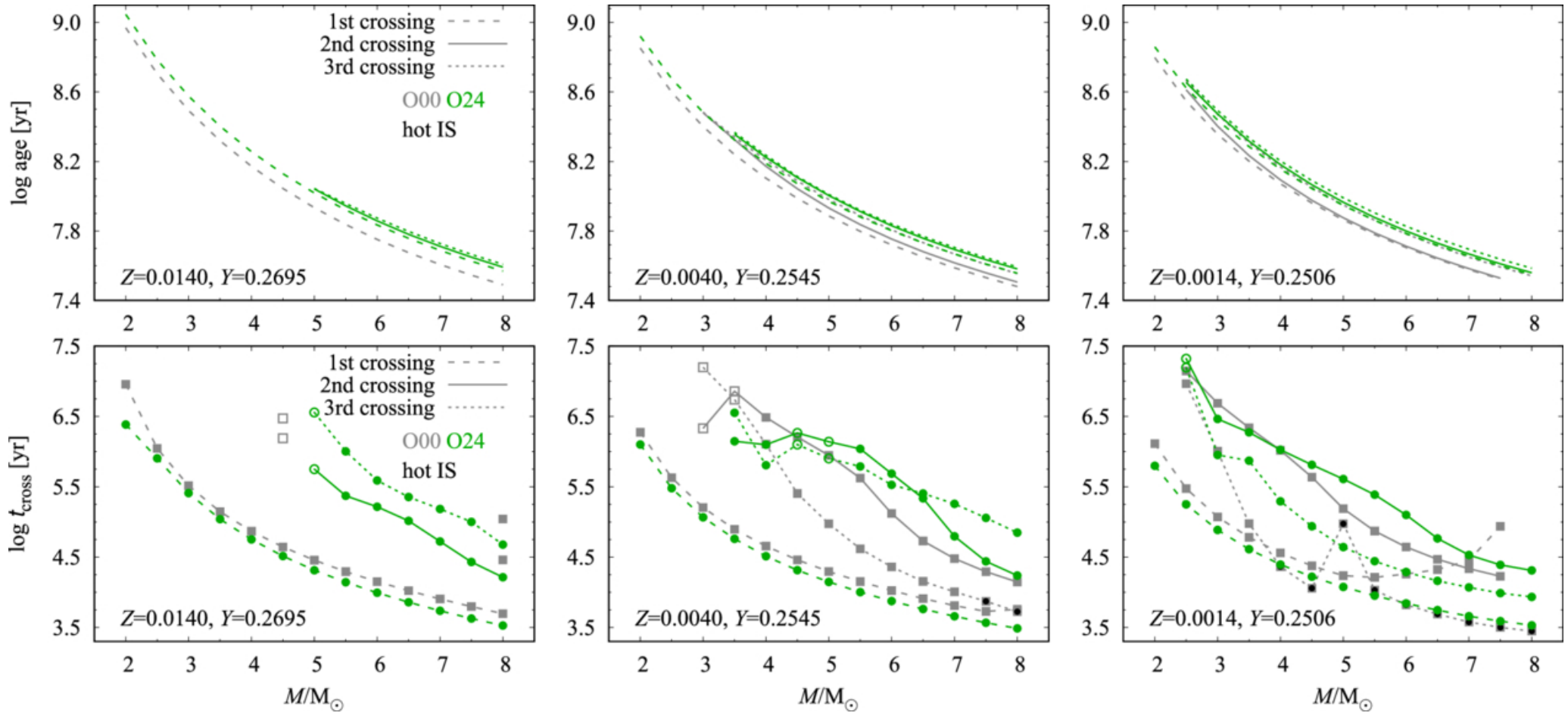
Figure 6. from Radoslaw Smolec et al 2026 Astrophys. J. Suppl. 284 doi:10.3847/1538-4365/ae6073 https://dx.doi.org/10.3847/1538-4365/ae6073 © 2026. The Author(s). Published by the American Astronomical Society.
