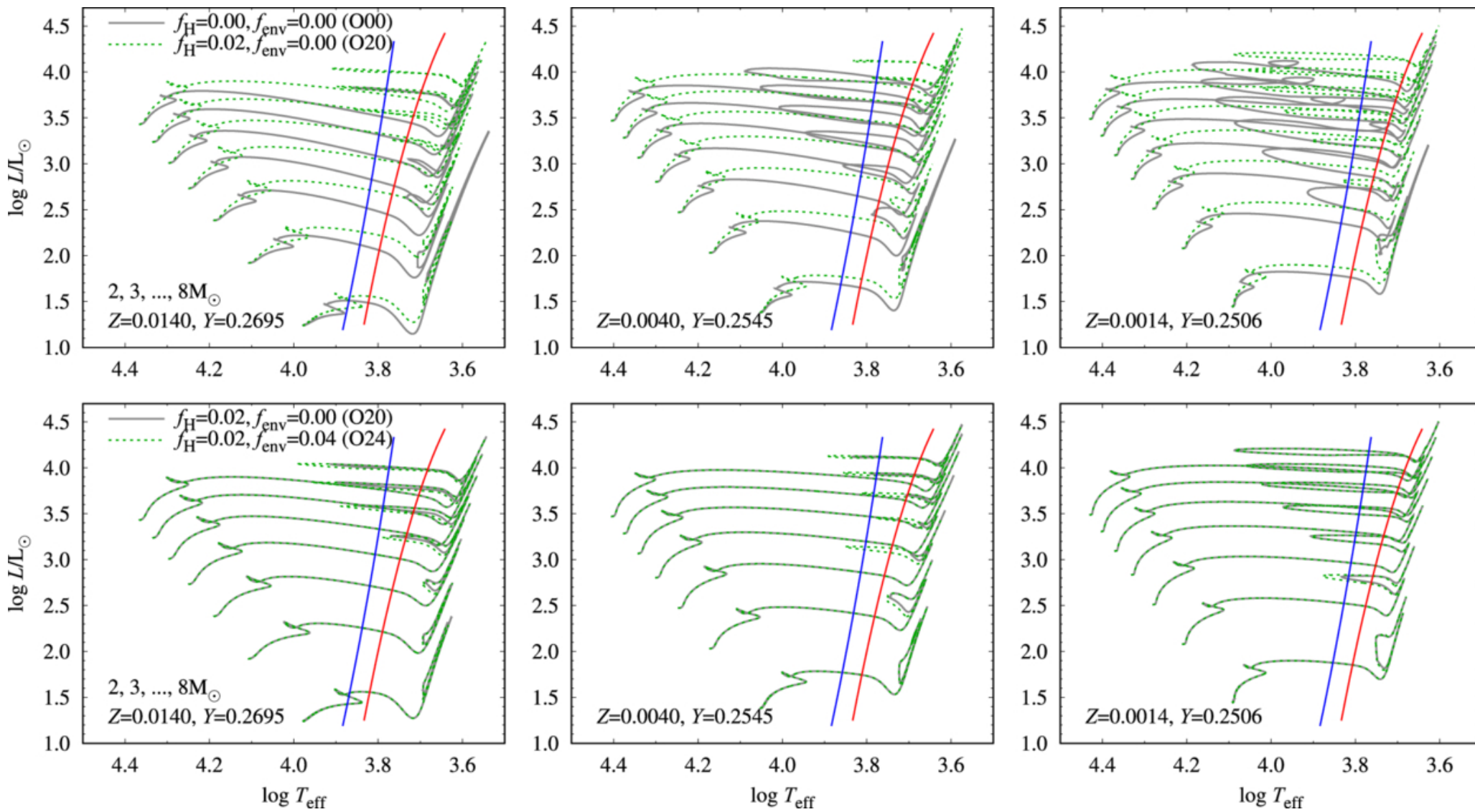
Figure 3. from Radoslaw Smolec et al 2026 Astrophys. J. Suppl. 284 doi:10.3847/1538-4365/ae6073 https://dx.doi.org/10.3847/1538-4365/ae6073 © 2026. The Author(s). Published by the American Astronomical Society.
