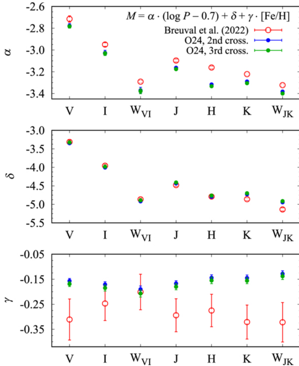
Figure 10. from Radoslaw Smolec et al 2026 Astrophys. J. Suppl. 284 doi:10.3847/1538-4365/ae6073 https://dx.doi.org/10.3847/1538-4365/ae6073 © 2026. The Author(s). Published by the American Astronomical Society.
