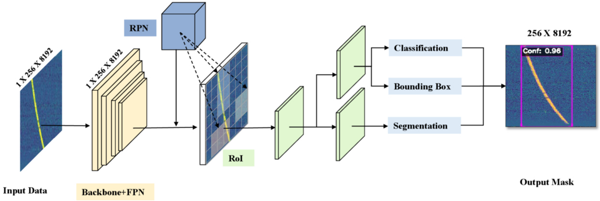
Figure 5. from Bin Zhang et al 2026 Astrophys. J. Suppl. 284 doi:10.3847/1538-4365/ae5e76 https://dx.doi.org/10.3847/1538-4365/ae5e76 © 2026. The Author(s). Published by the American Astronomical Society.
