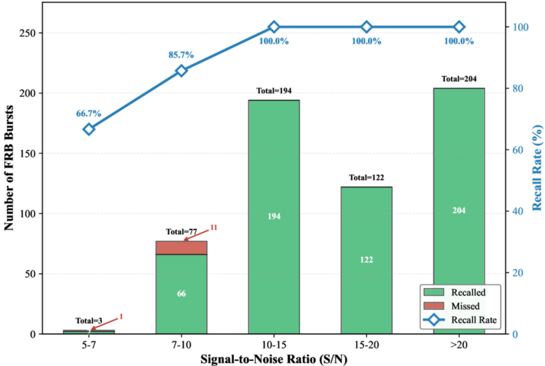
Figure 10. from Bin Zhang et al 2026 Astrophys. J. Suppl. 284 doi:10.3847/1538-4365/ae5e76 https://dx.doi.org/10.3847/1538-4365/ae5e76 © 2026. The Author(s). Published by the American Astronomical Society.
