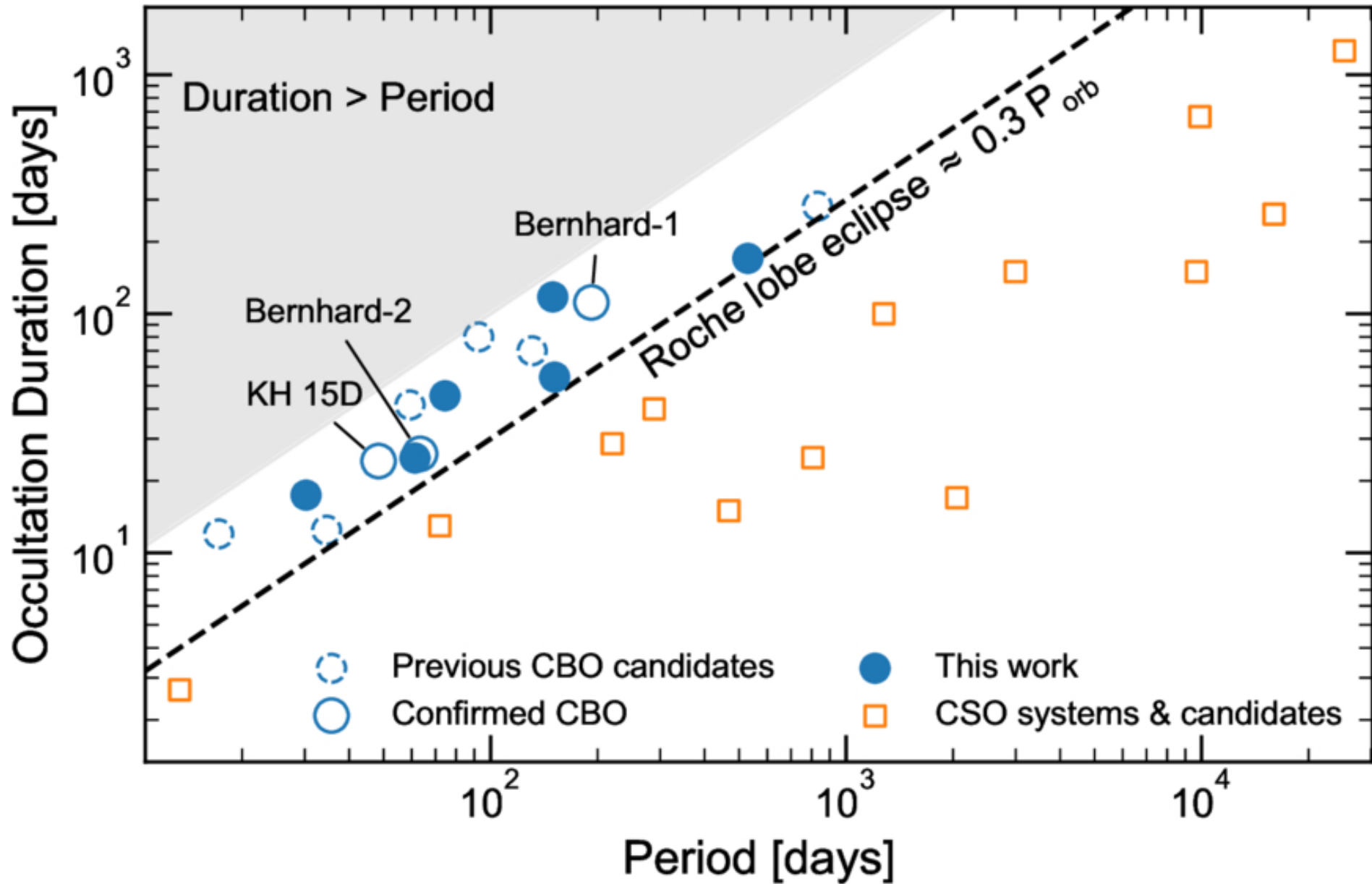
Figure 8. from Zhecheng Hu et al 2026 Astrophys. J. Suppl. 284 doi:10.3847/1538-4365/ae5d41 https://dx.doi.org/10.3847/1538-4365/ae5d41 © 2026. The Author(s). Published by the American Astronomical Society.
