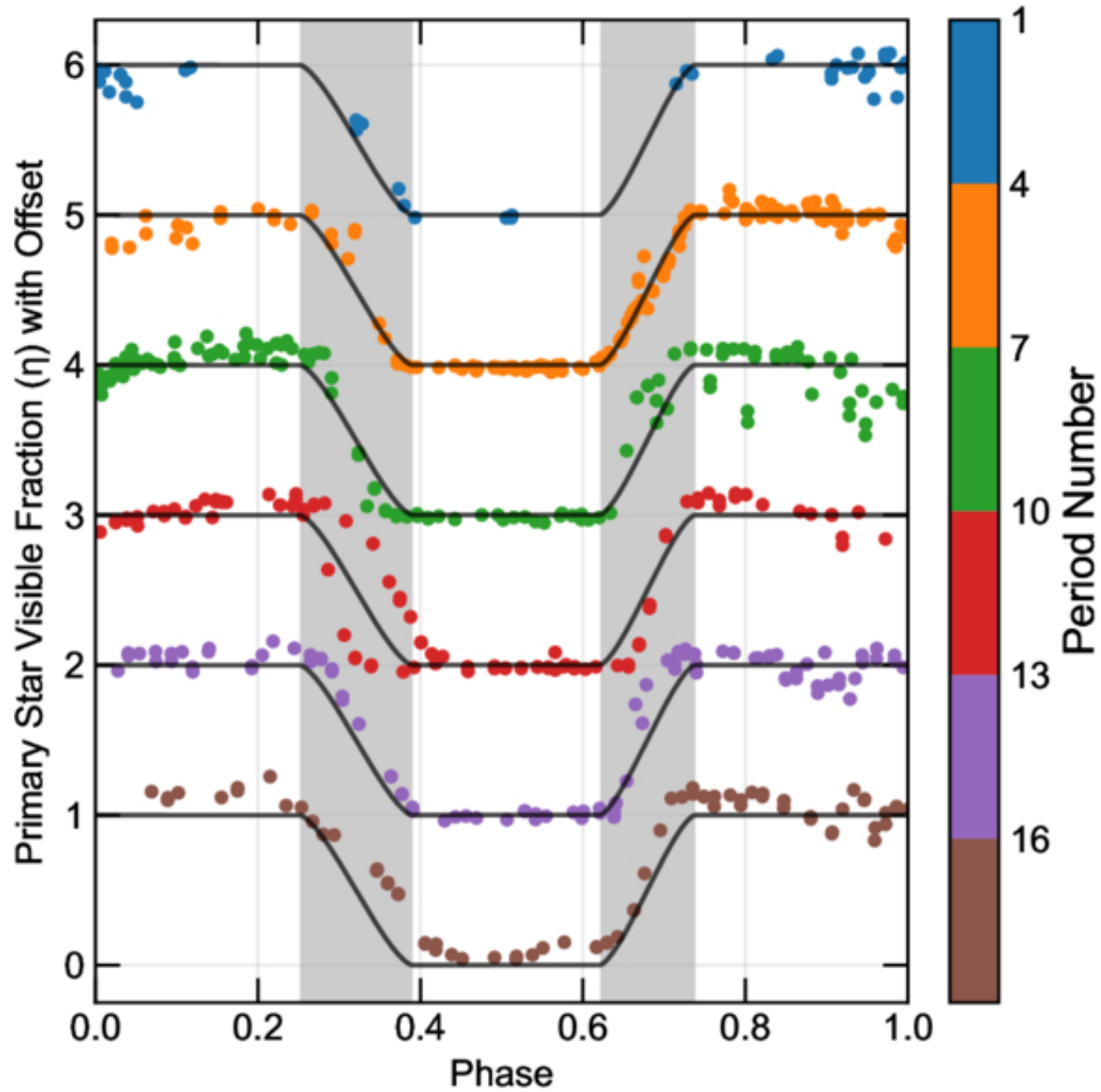
Figure 6. from Zhecheng Hu et al 2026 Astrophys. J. Suppl. 284 doi:10.3847/1538-4365/ae5d41 https://dx.doi.org/10.3847/1538-4365/ae5d41 © 2026. The Author(s). Published by the American Astronomical Society.
