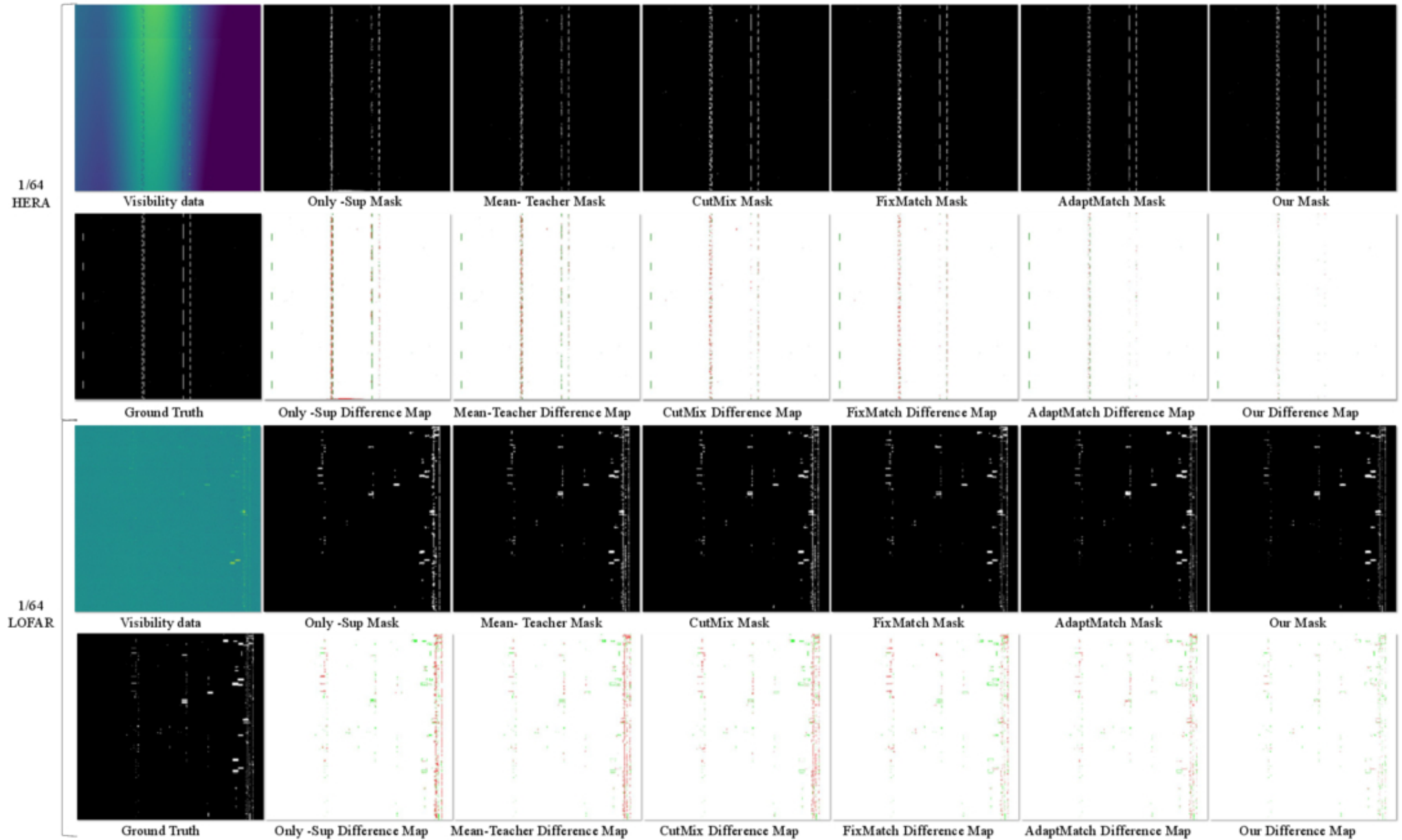
Figure 8. from Suxun Zhu et al 2026 Astrophys. J. Suppl. 284 doi:10.3847/1538-4365/ae5d39 https://dx.doi.org/10.3847/1538-4365/ae5d39 © 2026. The Author(s). Published by the American Astronomical Society.
