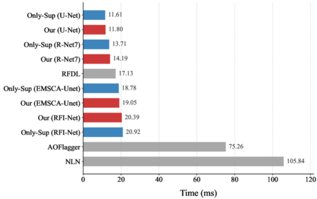
(a) HERA
