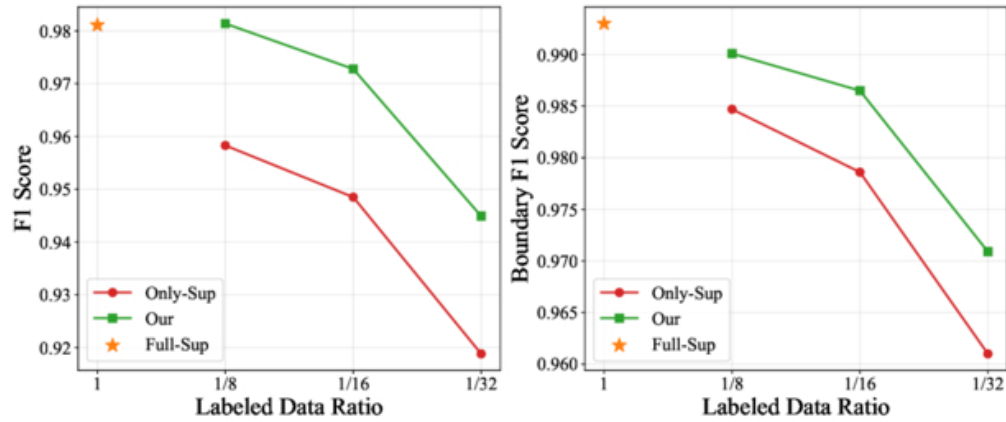
(a) EMSCA-Unet
