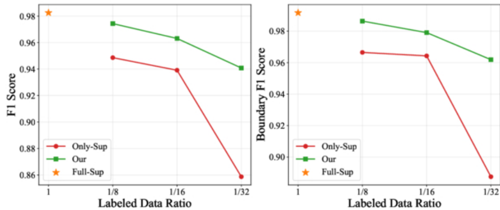
(c) R-Net7
