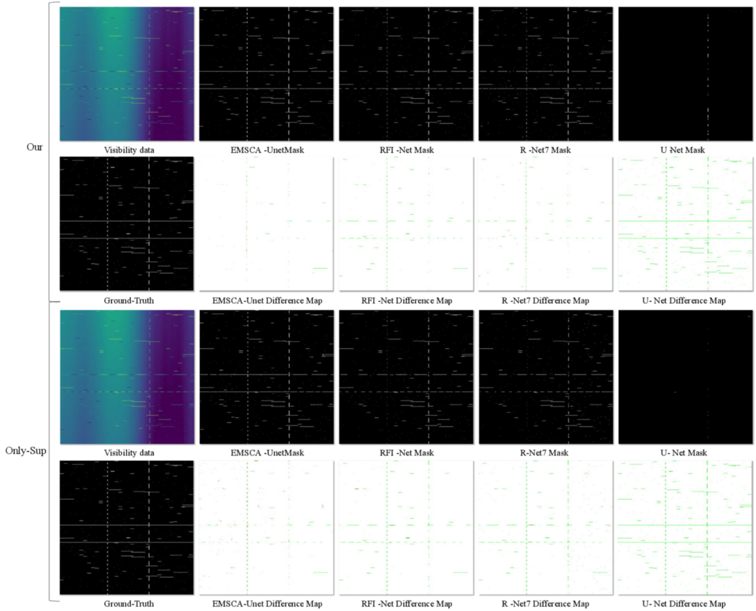
Figure 3. from Suxun Zhu et al 2026 Astrophys. J. Suppl. 284 doi:10.3847/1538-4365/ae5d39 https://dx.doi.org/10.3847/1538-4365/ae5d39 © 2026. The Author(s). Published by the American Astronomical Society.
